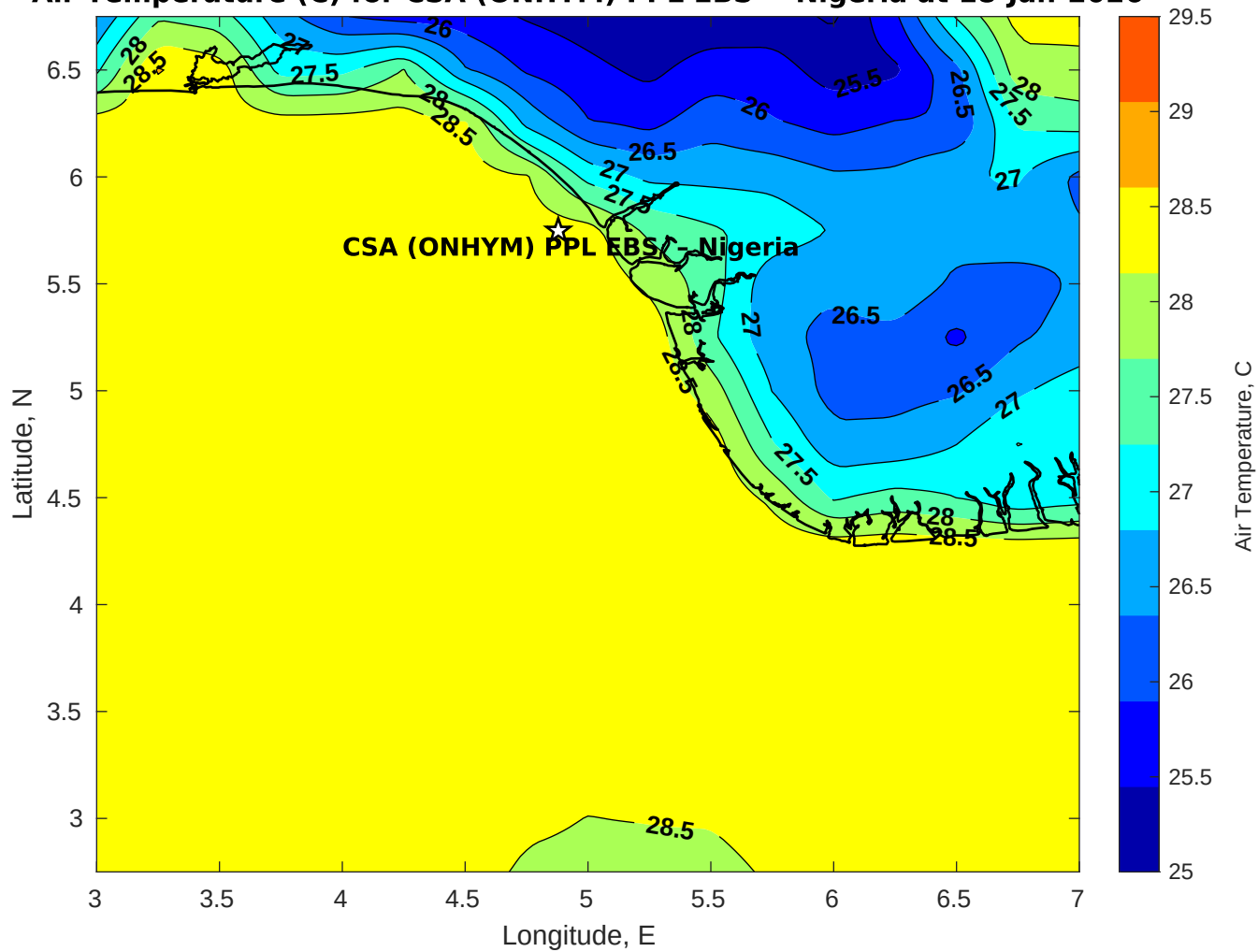
Air Temperature (C) for CSA (ONHYM) PPL EBS - Nigeria at 18-Jan-2026
