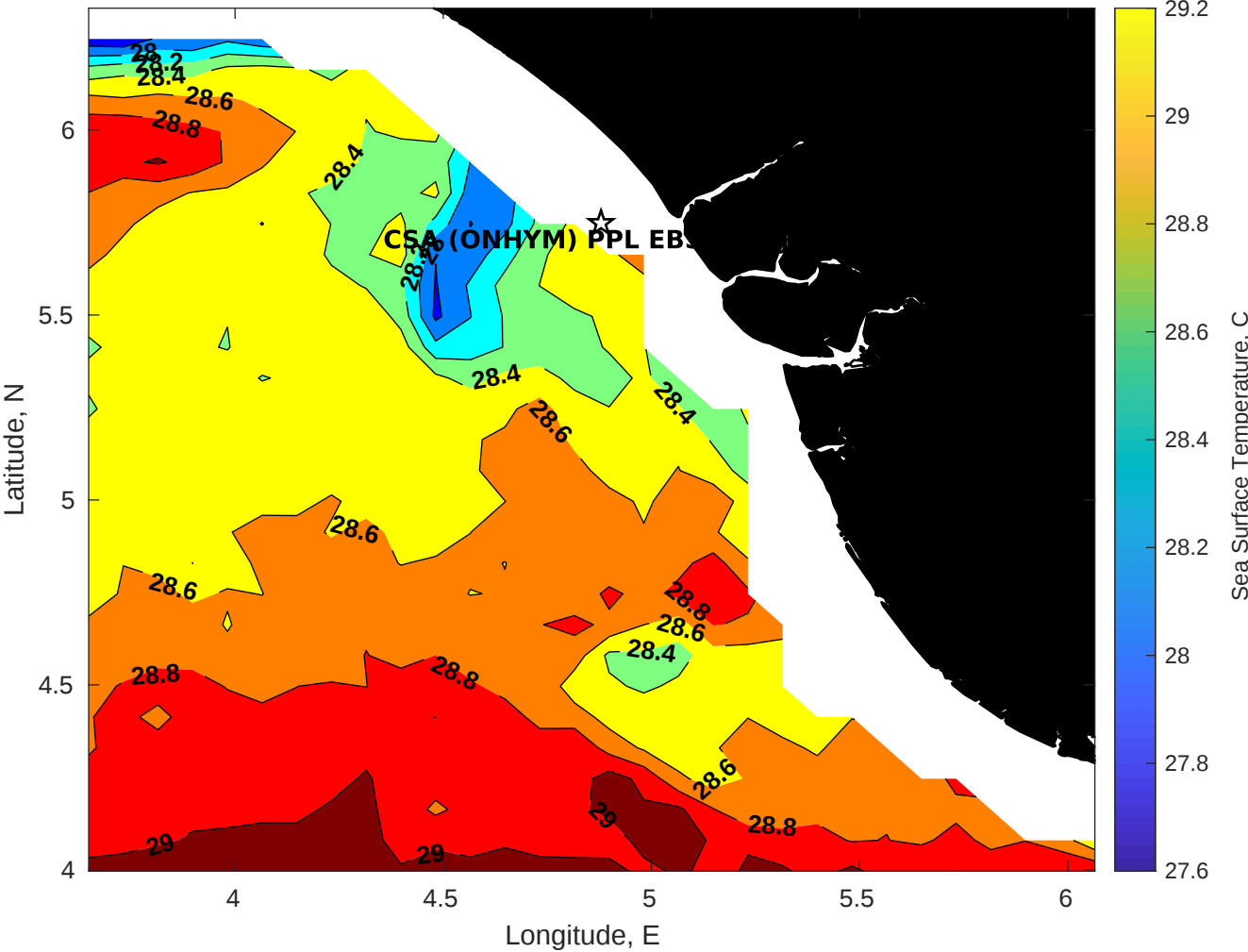
SST for CSA (ONHYM) PPL EBS - Nigeria at 17-Jan-2026 00:00:00
