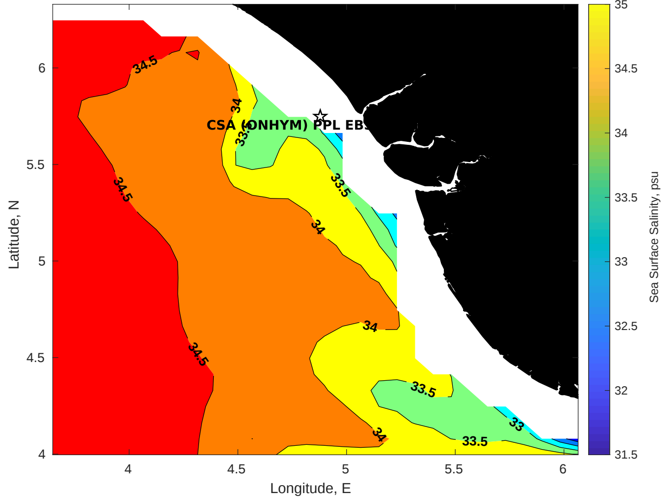
Surface Salinity for CSA (ONHYM) PPL EBS - Nigeria at 17-Jan-2026 00:00:00
