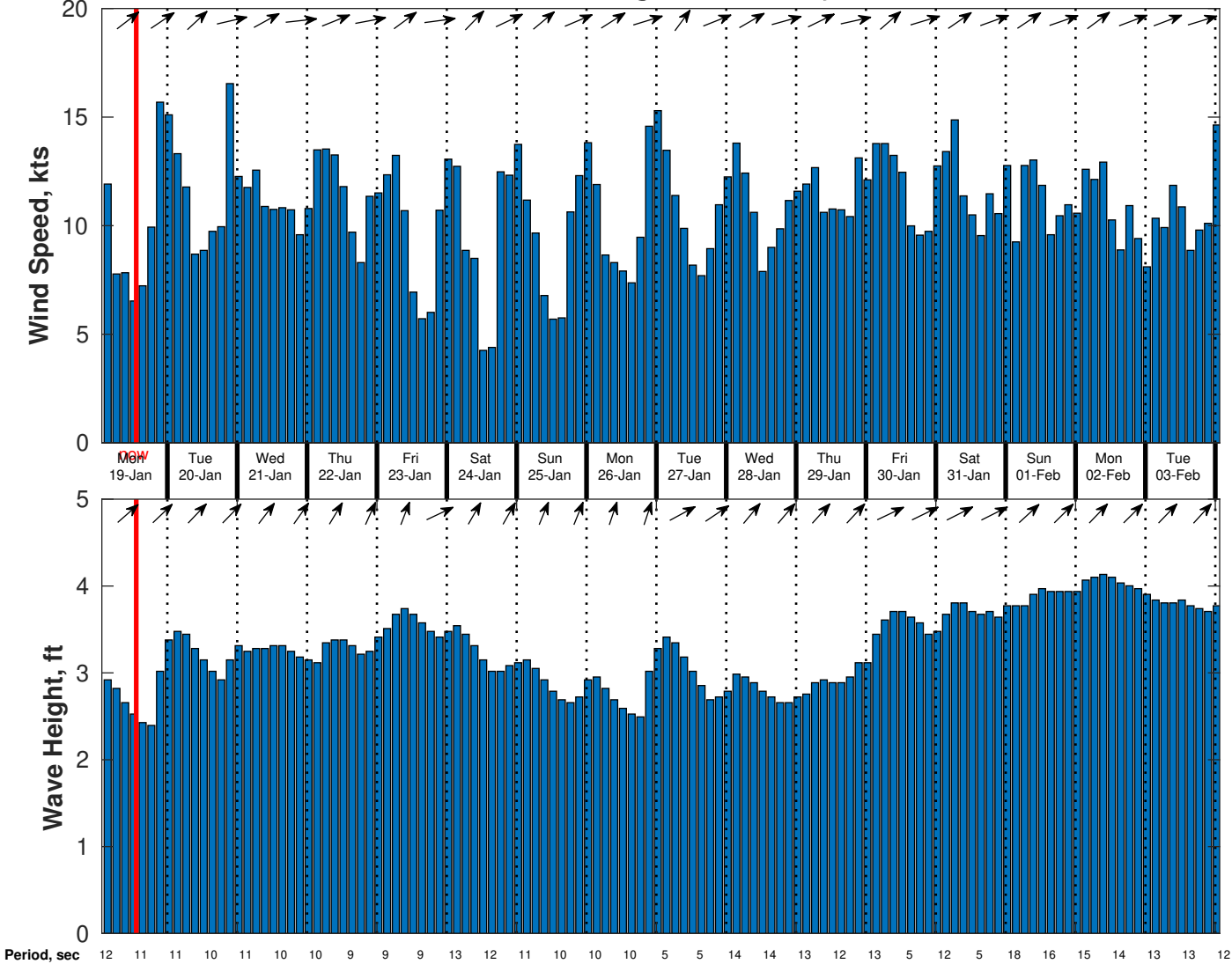
Wind & Wave Forecast for CSA (ONHYM) PPL EBS - Nigeria from 18-Jan-2026 02:00:00 to 03-Feb-2026 02:00:00
