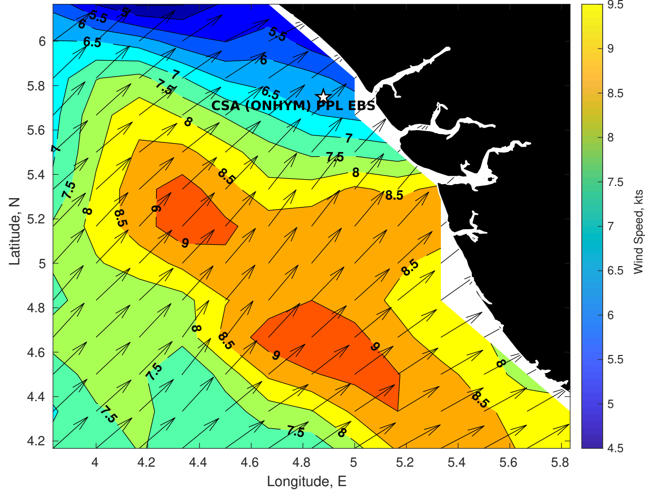
GFS Winds (kts) for CSA (ONHYM) PPL EBS - Nigeria at 18-Jan-2026 09:00:00
