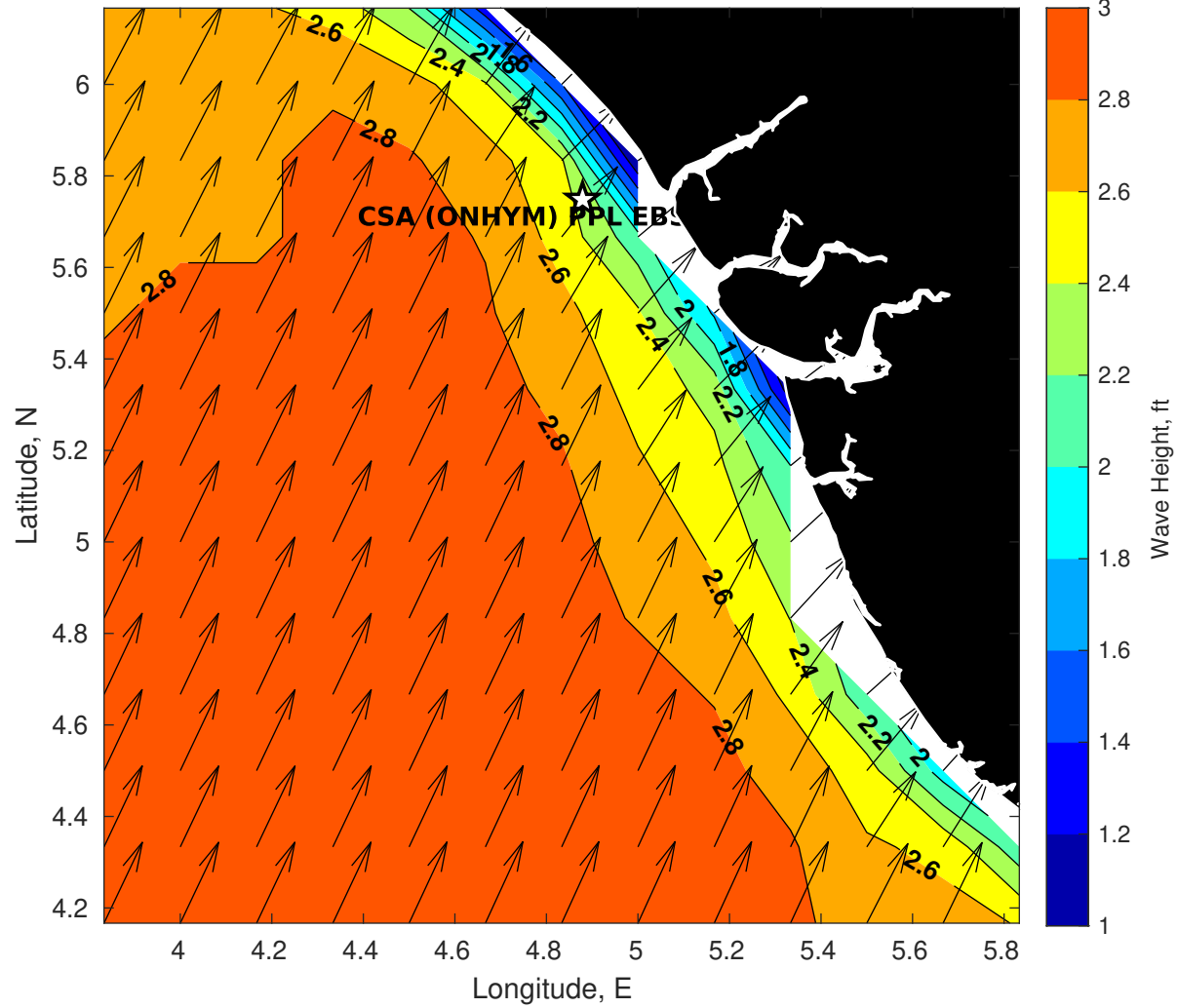
GFS Wave Height (ft) for CSA (ONHYM) PPL EBS - Nigeria at 18-Jan-2026 09:00:00
