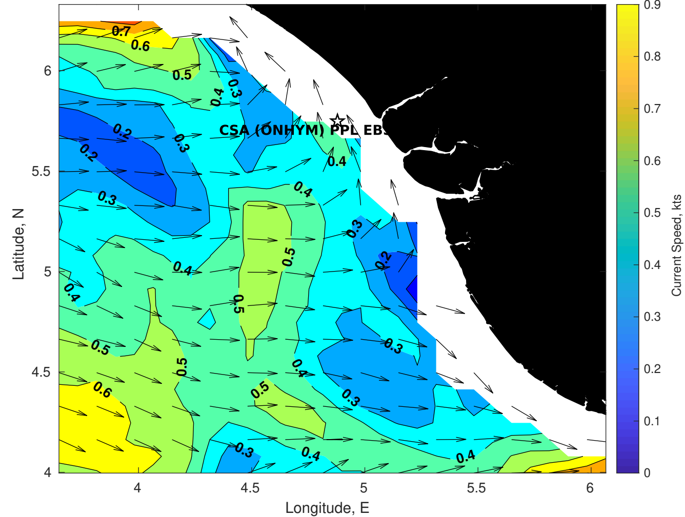
Surface Currents for CSA (ONHYM) PPL EBS - Nigeria at 17-Jan-2026 00:00:00
