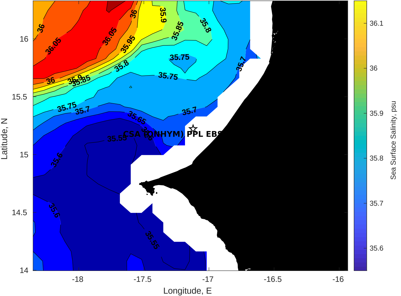
Surface Salinity for CSA (ONHYM) PPL EBS - Senegal at 17-Jan-2026 00:00:00
