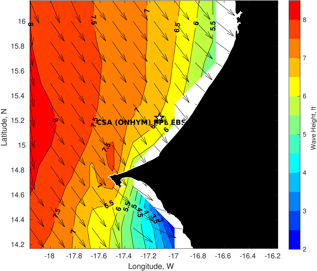
GFS Wave Height (ft) for CSA (ONHYM) PPL EBS - Senegal at 18-Jan-2026 09:00:00
