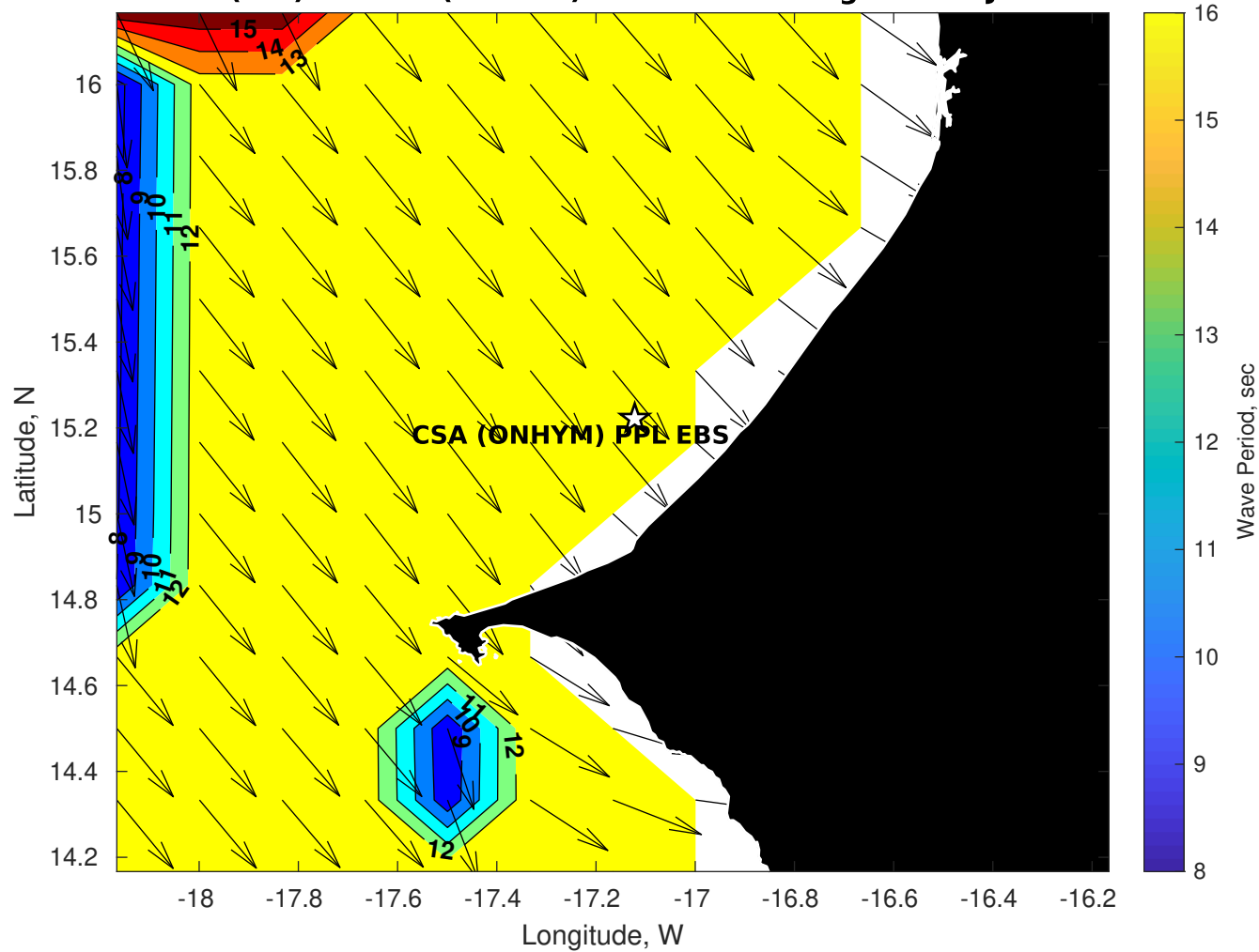
GFS Wave Period (sec) for CSA (ONHYM) PPL EBS - Senegal at 18-Jan-2026 09:00:00
