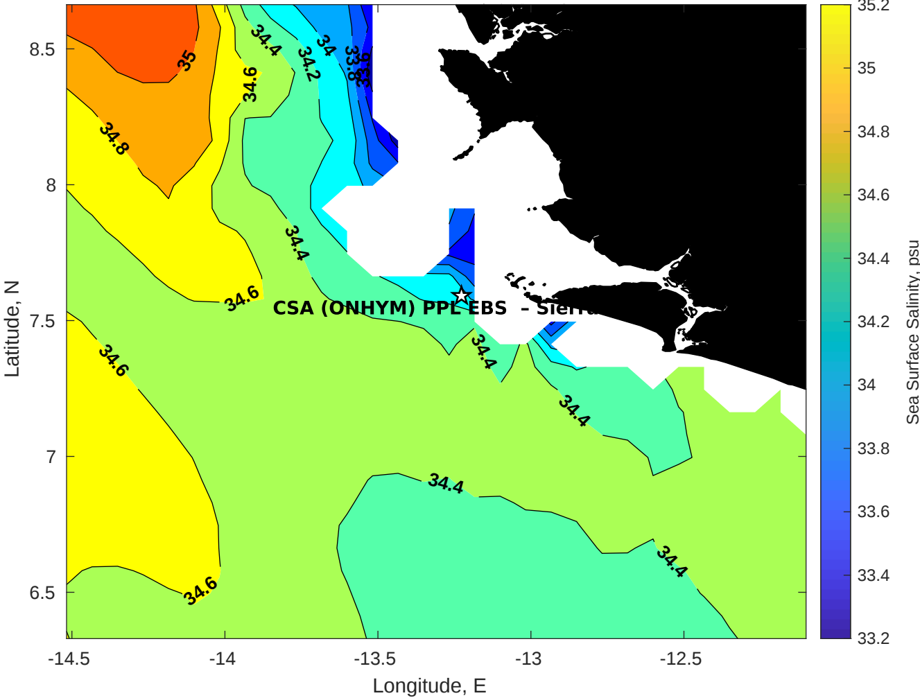
Surface Salinity for CSA (ONHYM) PPL EBS - Sierra Leone at 17-Jan-2026 00:00:00
