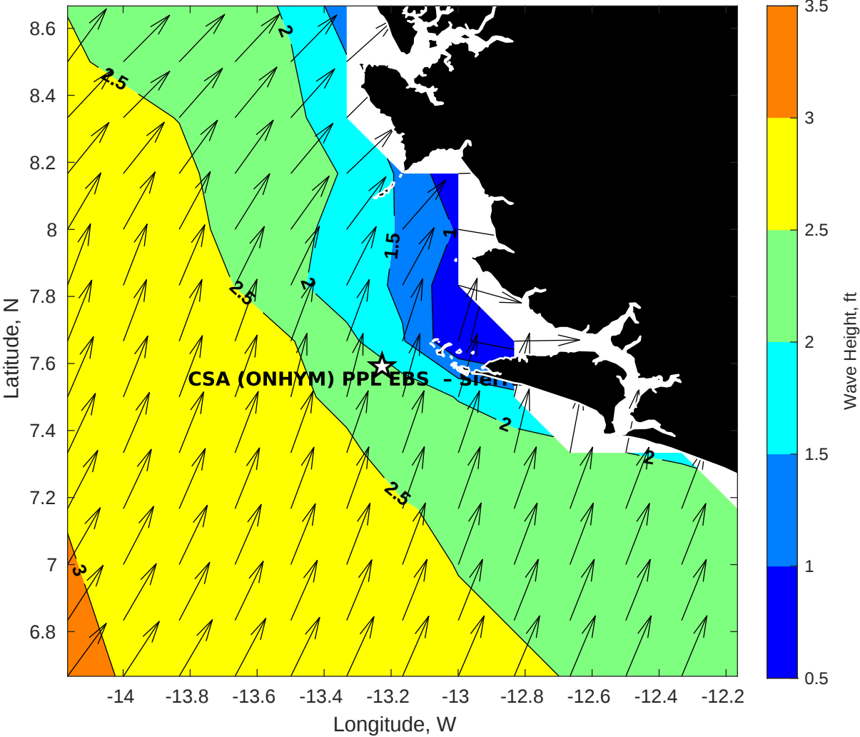
GFS Wave Height (ft) for CSA (ONHYM) PPL EBS - Sierra Leone at 18-Jan-2026 09:00:00
