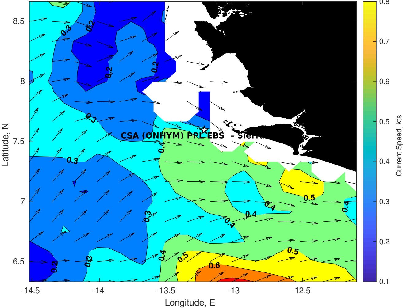
Surface Currents for CSA (ONHYM) PPL EBS - Sierra Leone at 17-Jan-2026 00:00:00
