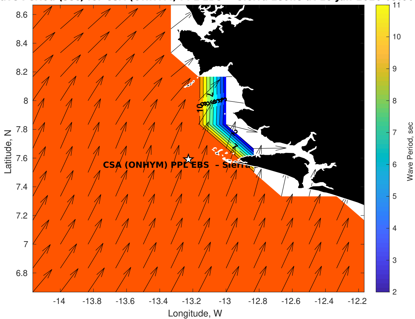
GFS Wave Period (sec) for CSA (ONHYM) PPL EBS - Sierra Leone at 18-Jan-2026 09:00:00
