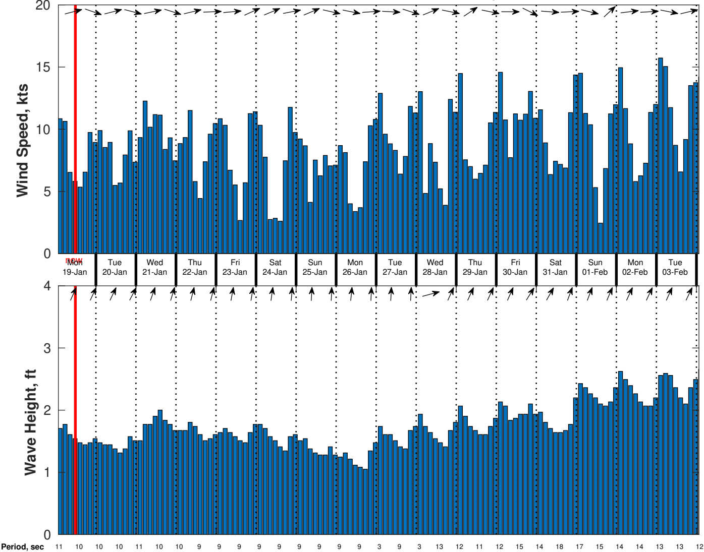
Wind & Wave Forecast for CSA (ONHYM) PPL EBS - Sierra Leone from 18-Jan-2026 01:00:00 to 03-Feb-2026 01:00:00
