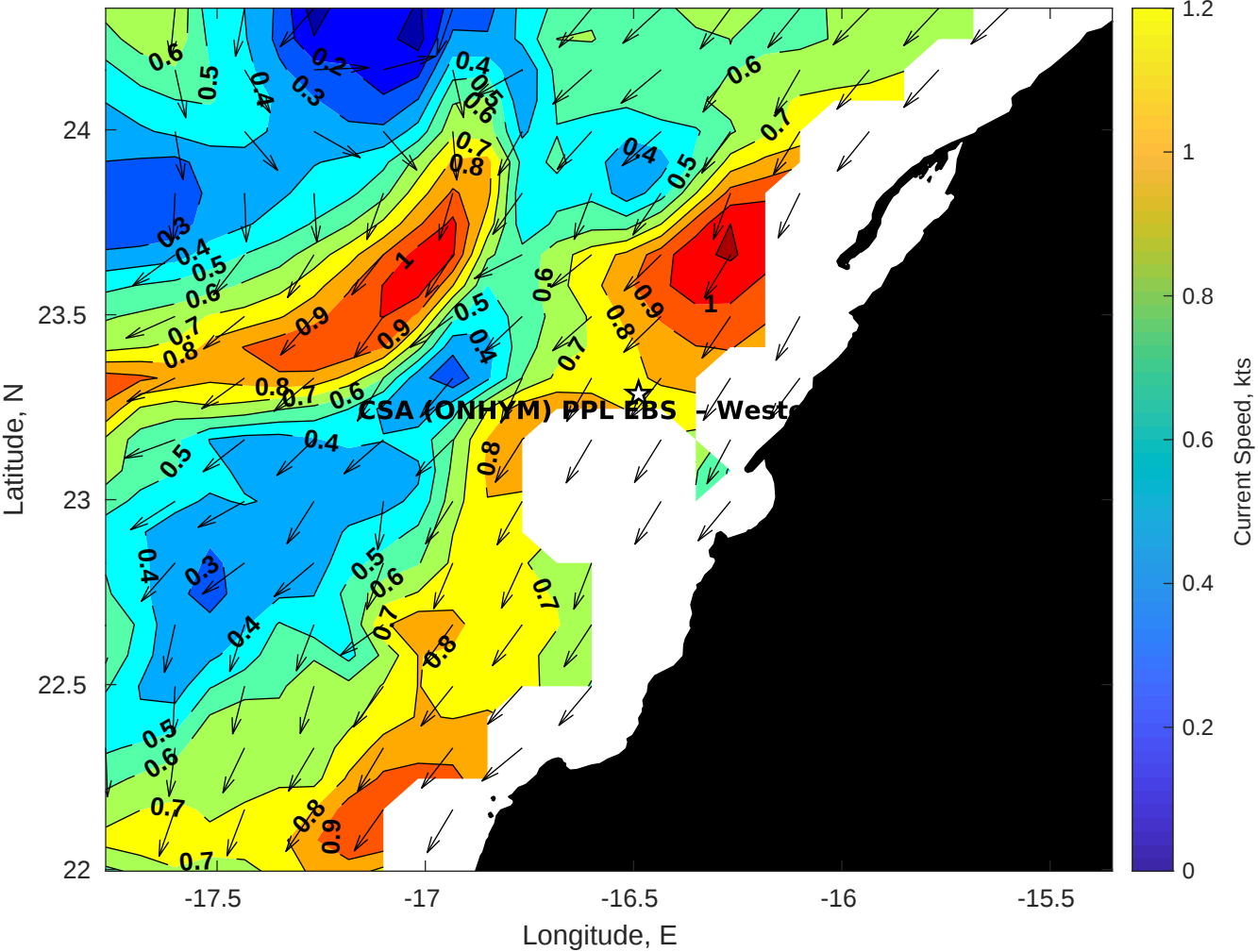
Surface Currents for CSA (ONHYM) PPL EBS - Western Sahara at 17-Jan-2026 00:00:00
