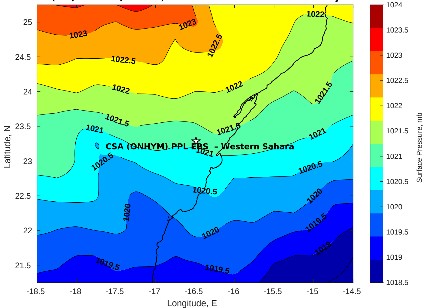
Surface Pressure (mb) for CSA (ONHYM) PPL EBS - Western Sahara at 20-Jan-2026 00:00:00
