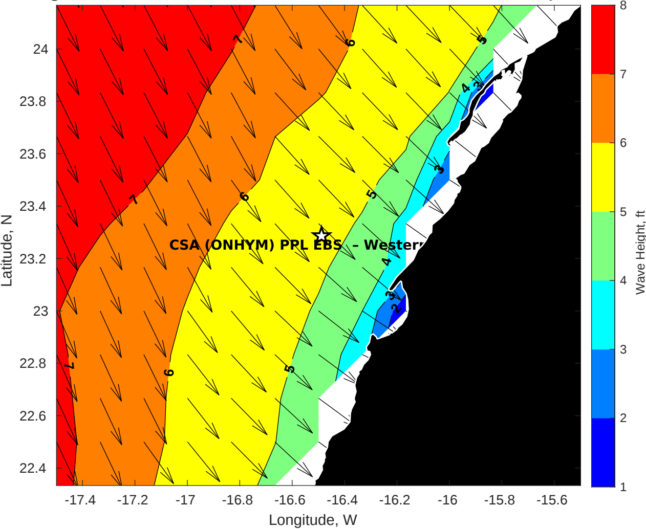
GFS Wave Height (ft) for CSA (ONHYM) PPL EBS - Western Sahara at 18-Jan-2026 09:00:00
