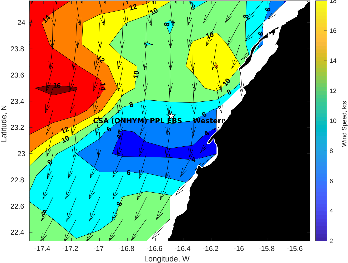
GFS Winds (kts) for CSA (ONHYM) PPL EBS - Western Sahara at 18-Jan-2026 09:00:00
