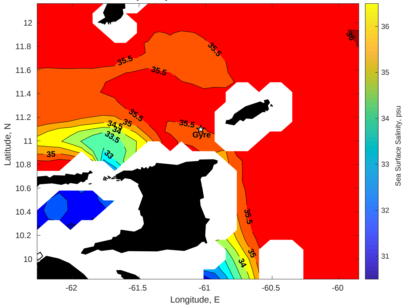
Surface Salinity for Gyre at 17-Jan-2026 00:00:00
