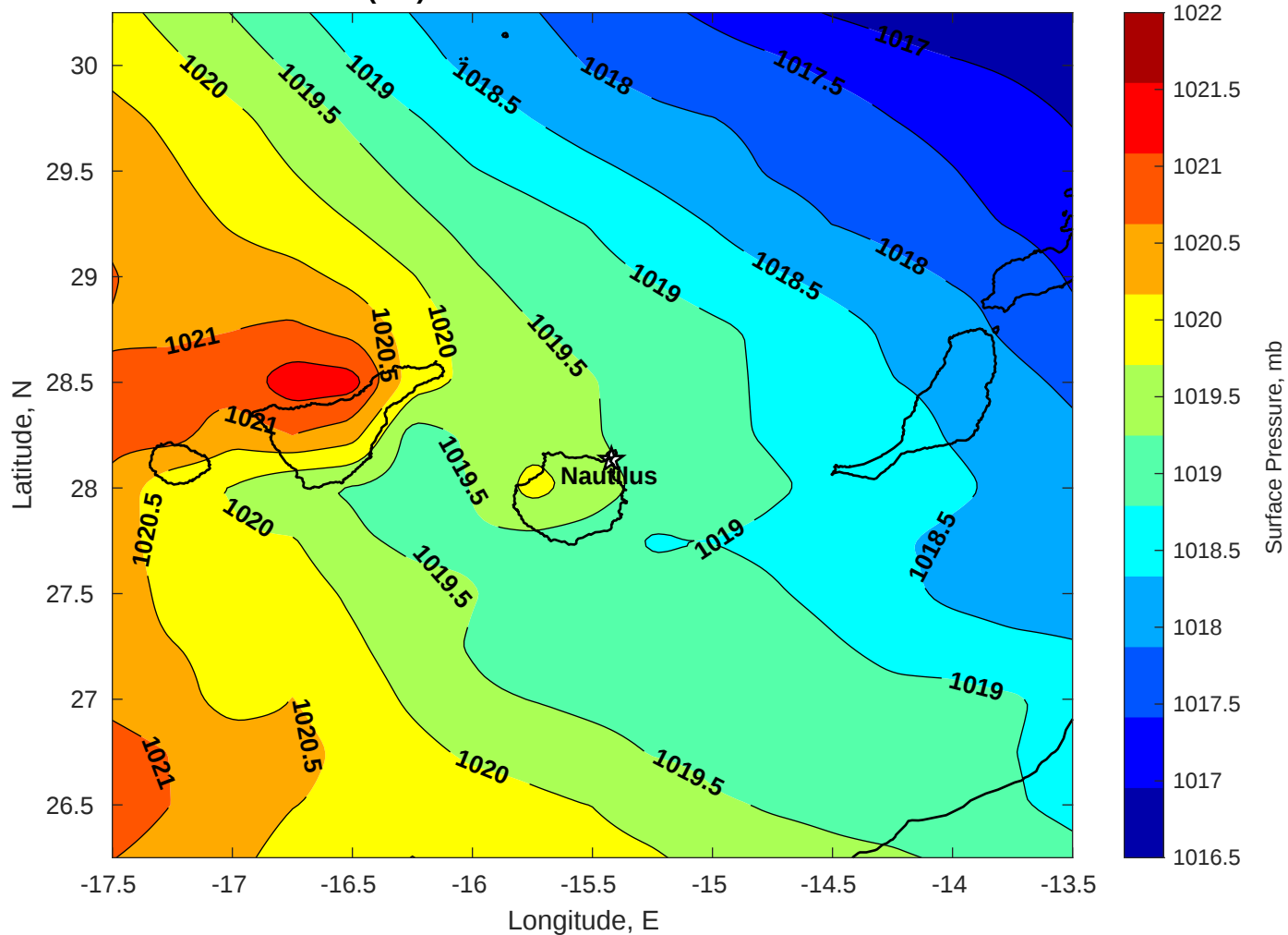
Surface Pressure (mb) for Nautilus at 18-Jan-2026 00:00:00
