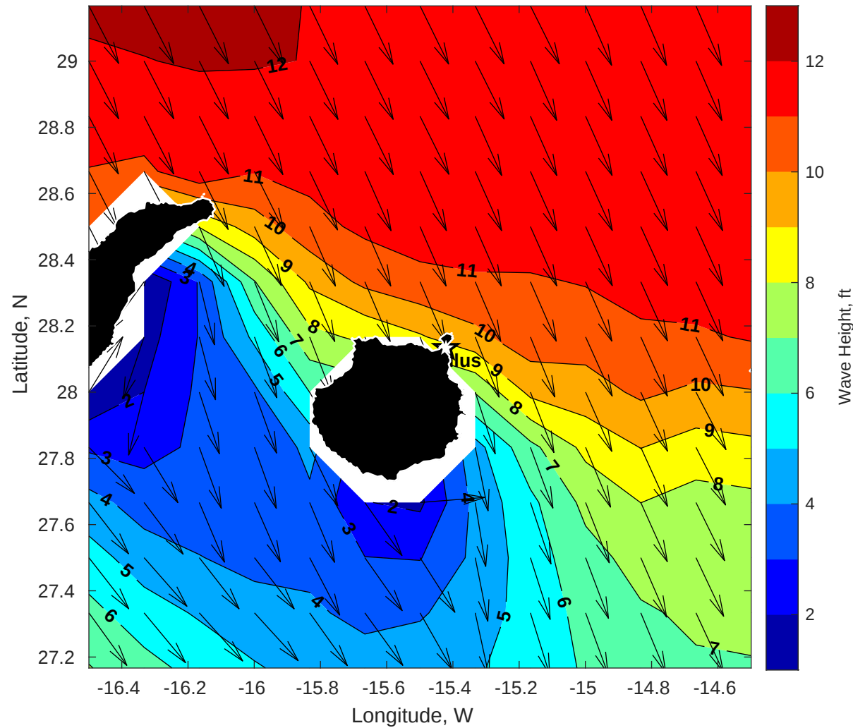
GFS Wave Height (ft) for Nautilus at 18-Jan-2026 09:00:00
