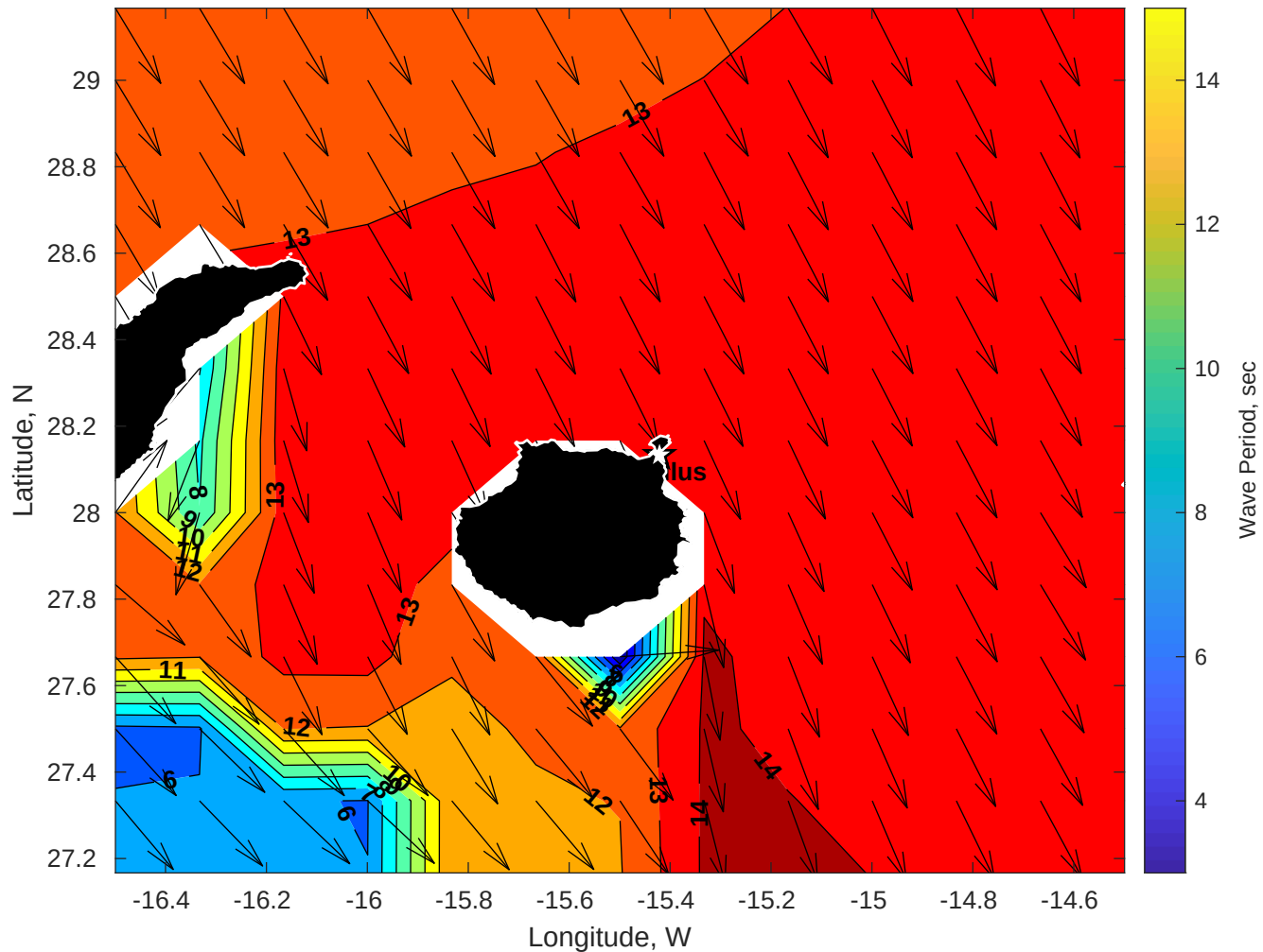
GFS Wave Period (sec) for Nautilus at 18-Jan-2026 09:00:00
