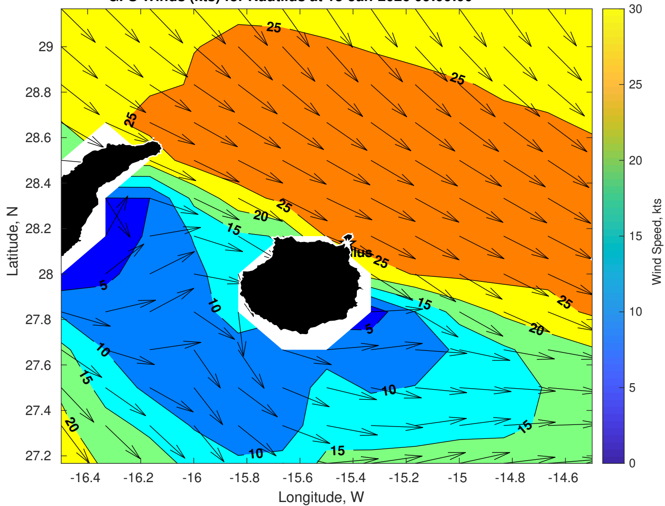
GFS Winds (kts) for Nautilus at 18-Jan-2026 09:00:00
