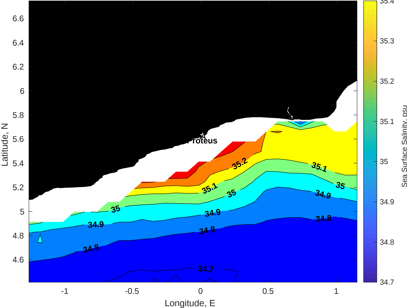
Surface Salinity for Proteus at 17-Jan-2026 00:00:00
