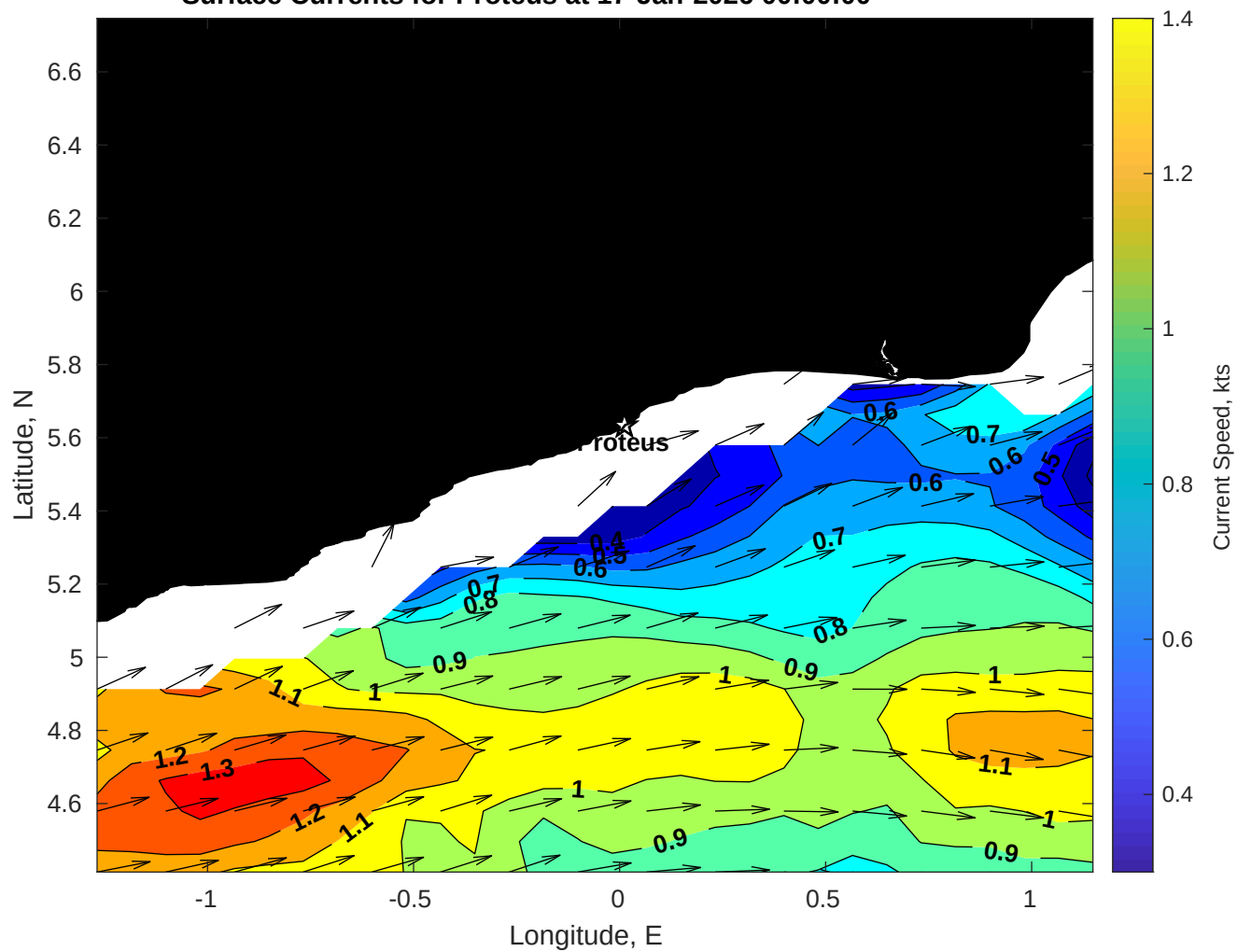
Surface Currents for Proteus at 17-Jan-2026 00:00:00
