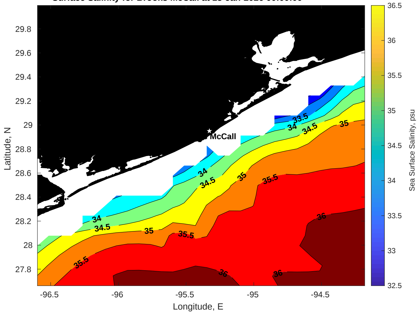
Surface Salinity for Brooks McCall at 18-Jan-2026 00:00:00
