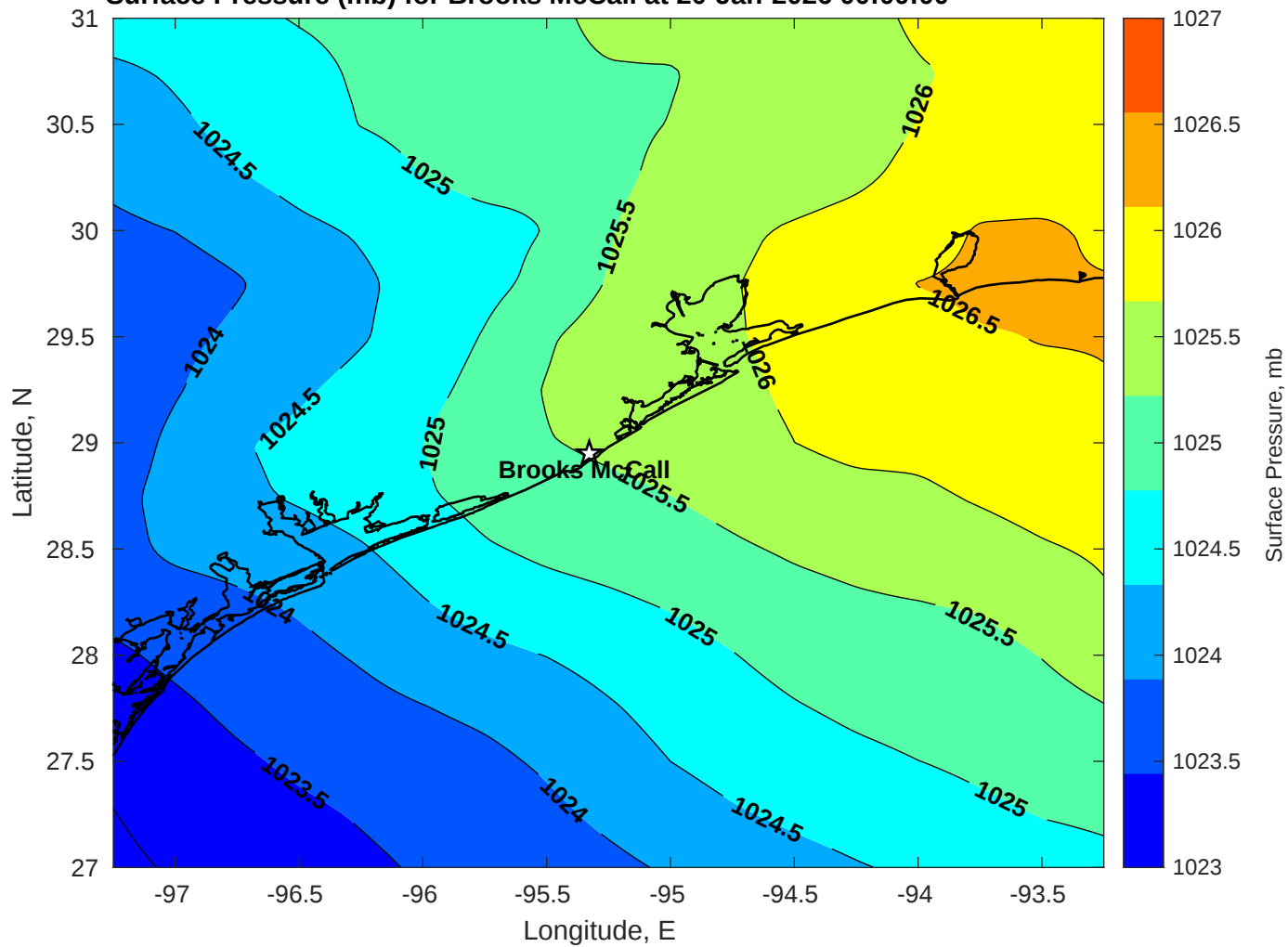
Surface Pressure (mb) for Brooks McCall at 20-Jan-2026 00:00:00
