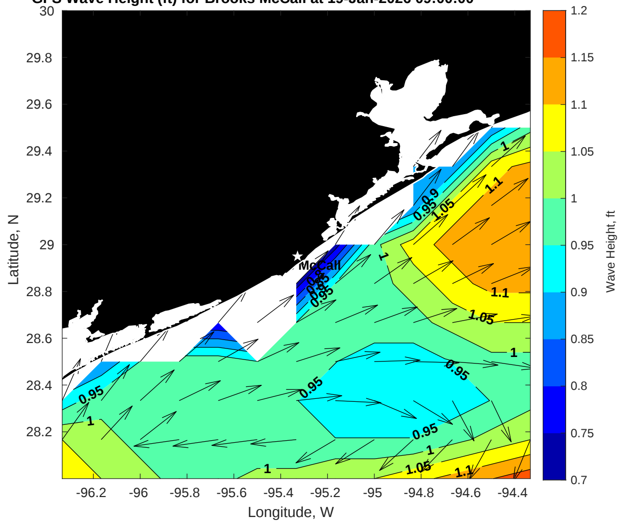
GFS Wave Height (ft) for Brooks McCall at 19-Jan-2026 09:00:00
