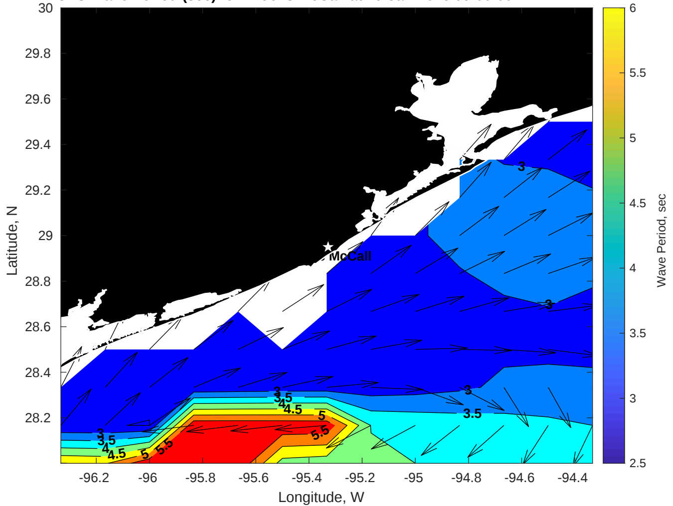
GFS Wave Period (sec) for Brooks McCall at 19-Jan-2026 09:00:00
