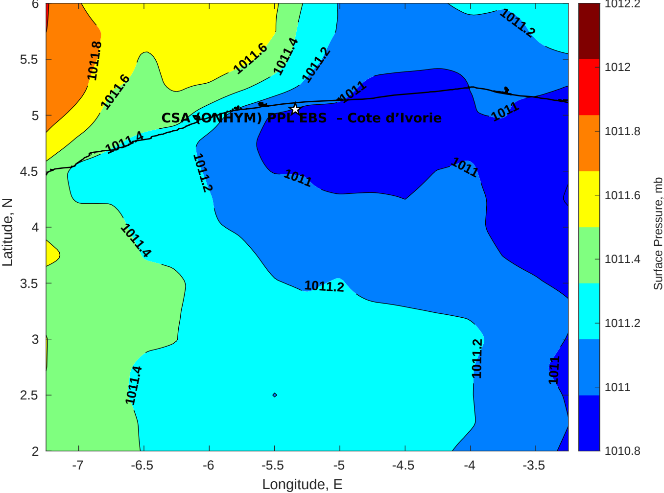
Surface Pressure (mb) for CSA (ONHYM) PPL EBS - Cote d'Ivoire at 21-Jan-2026 00:00:00
