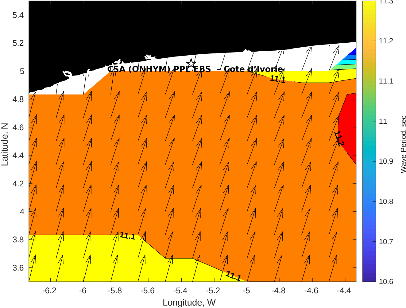
GFS Wave Period (sec) for CSA (ONHYM) PPL EBS - Cote d'Ivoire at 19-Jan-2026 09:00:00
