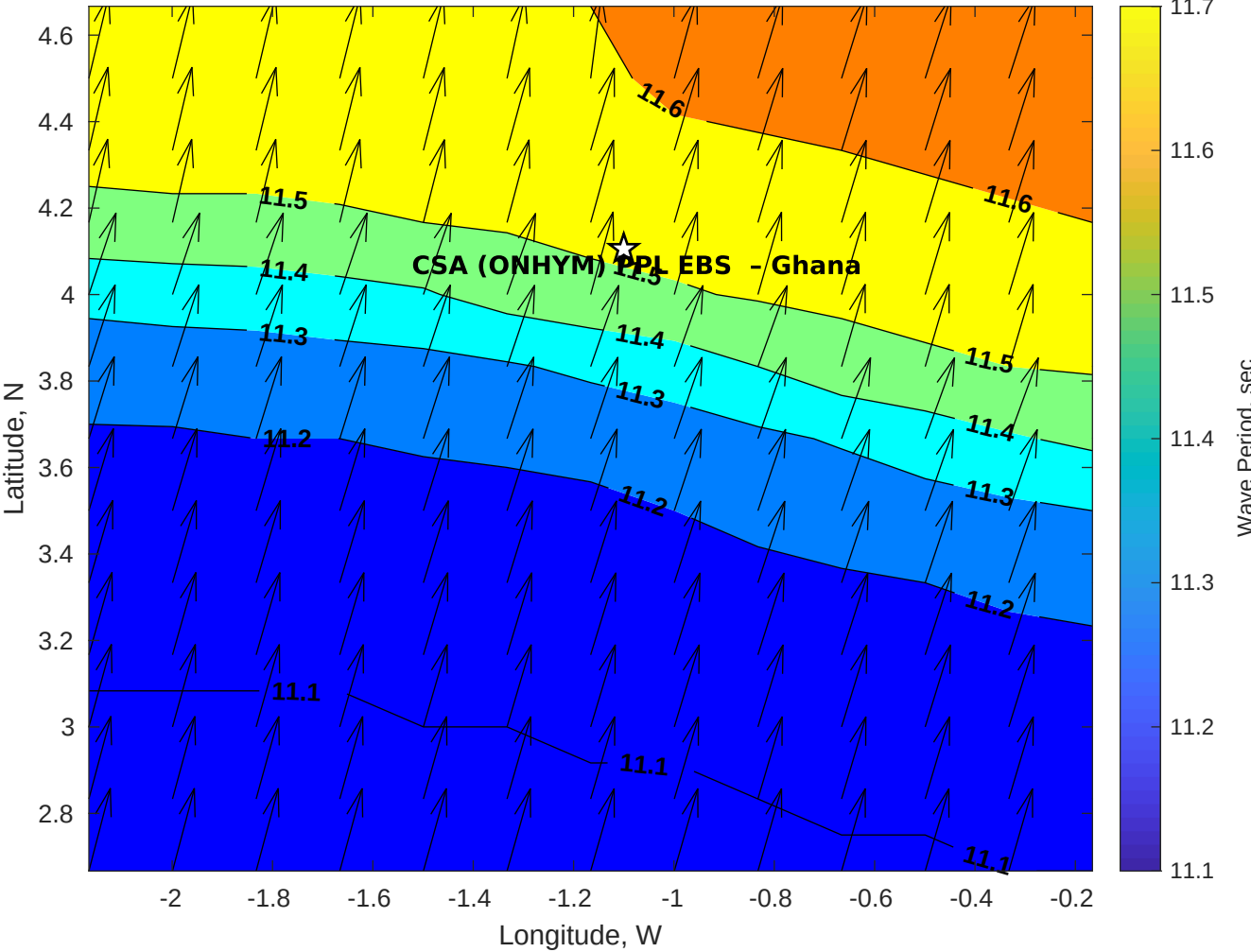
GFS Wave Period (sec) for CSA (ONHYM) PPL EBS - Ghana at 19-Jan-2026 09:00:00
