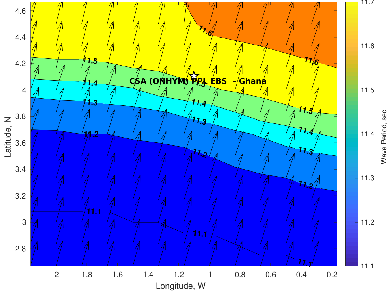
GFS Wave Period (sec) for CSA (ONHYM) PPL EBS - Ghana at 19-Jan-2026 09:00:00
