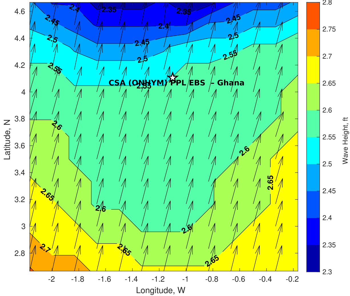
GFS Wave Height (ft) for CSA (ONHYM) PPL EBS - Ghana at 19-Jan-2026 09:00:00
