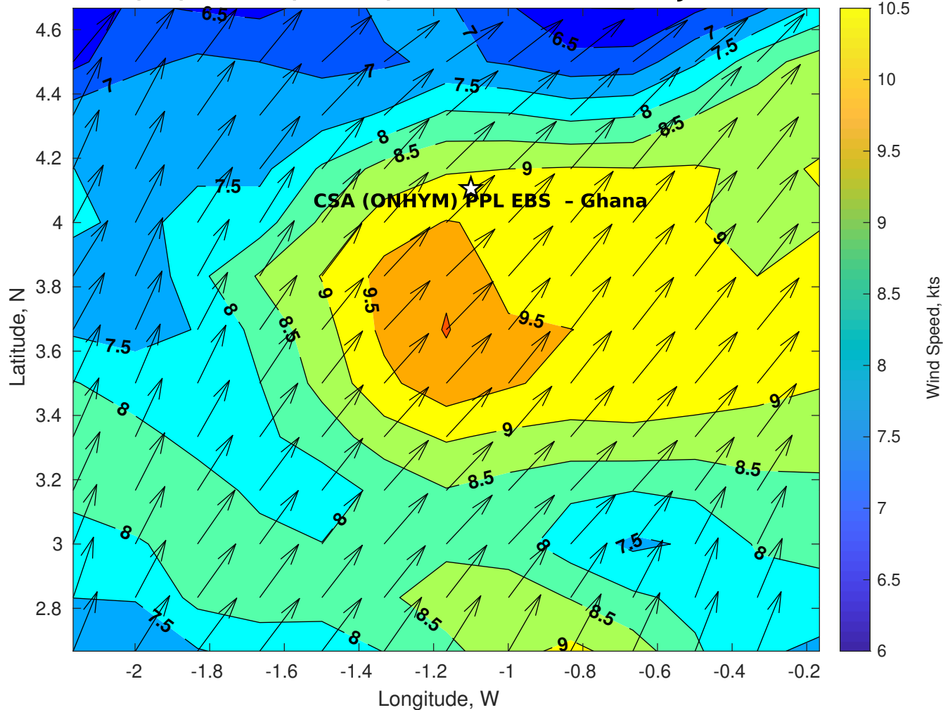
GFS Winds (kts) for CSA (ONHYM) PPL EBS - Ghana at 19-Jan-2026 09:00:00
