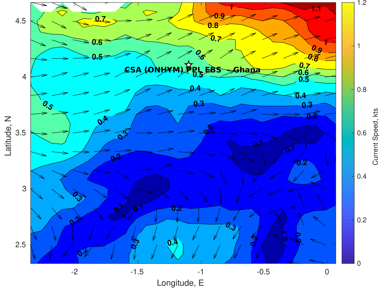
Surface Currents for CSA (ONHYM) PPL EBS - Ghana at 18-Jan-2026 00:00:00
