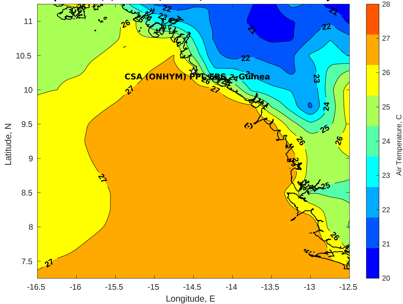
Air Temperature (C) for CSA (ONHYM) PPL EBS - Guinea at 19-Jan-2026
