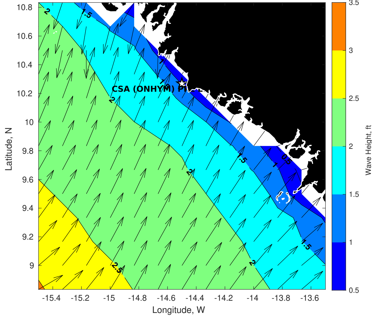
GFS Wave Height (ft) for CSA (ONHYM) PPL EBS - Guinea at 19-Jan-2026 09:00:00
