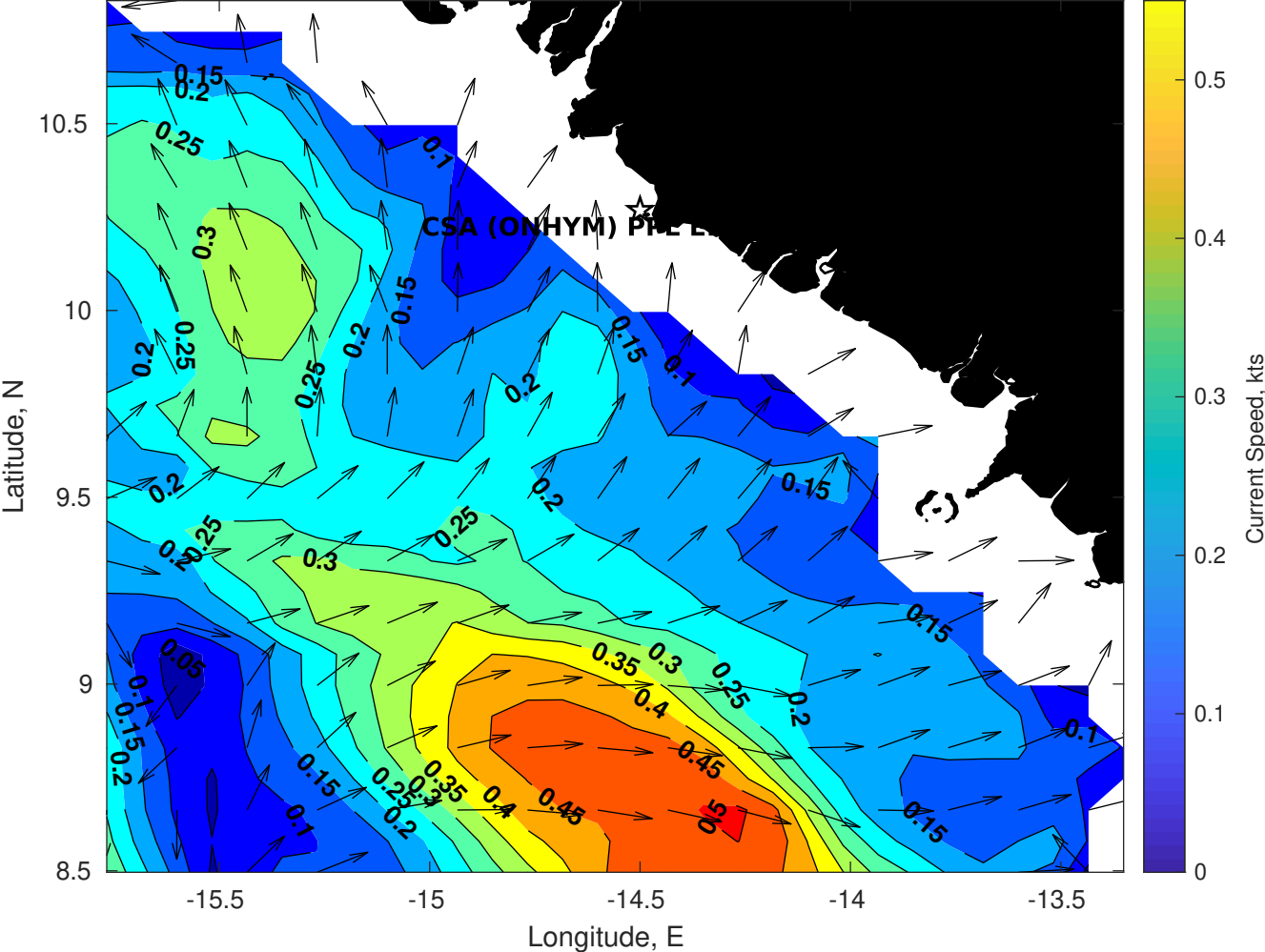
Surface Currents for CSA (ONHYM) PPL EBS - Guinea at 18-Jan-2026 00:00:00
