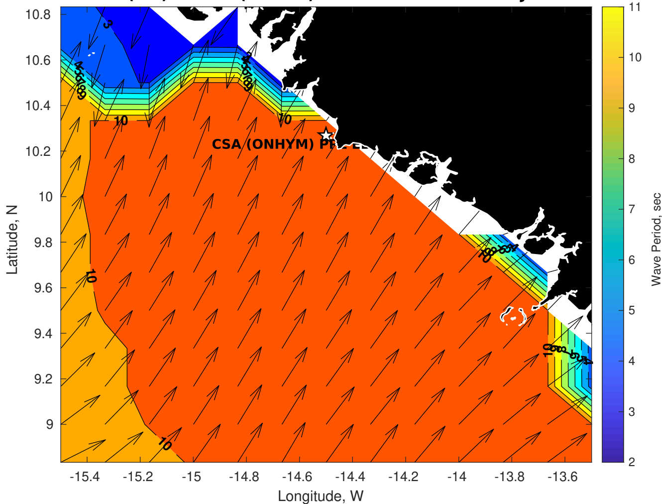
GFS Wave Period (sec) for CSA (ONHYM) PPL EBS - Guinea at 19-Jan-2026 09:00:00
