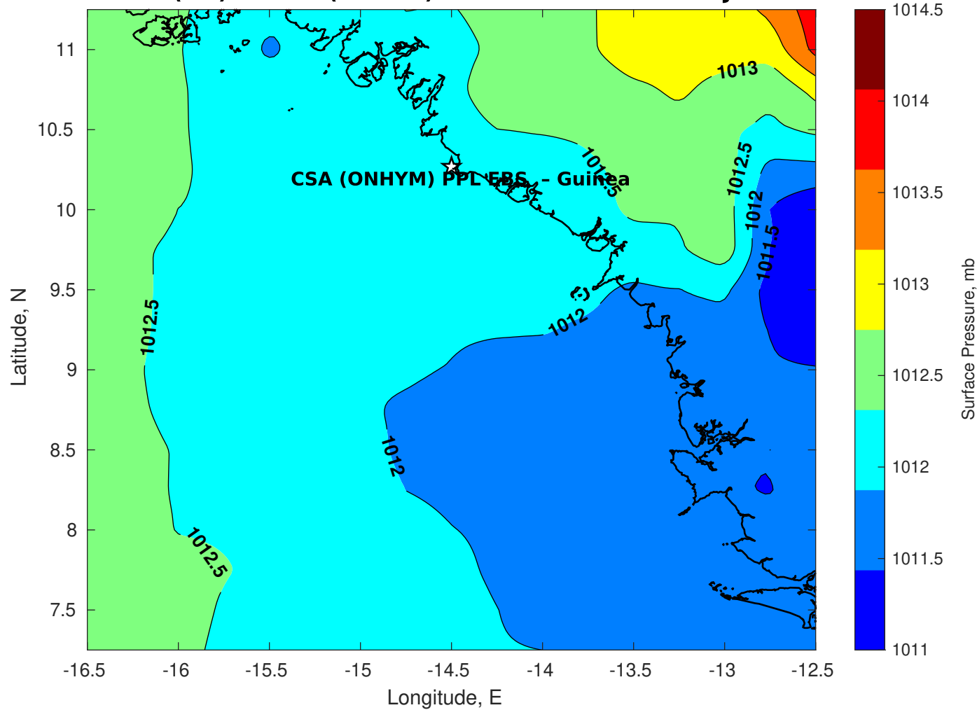
Surface Pressure (mb) for CSA (ONHYM) PPL EBS - Guinea at 21-Jan-2026 00:00:00
