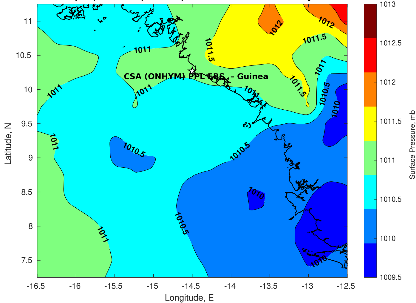
Surface Pressure (mb) for CSA (ONHYM) PPL EBS - Guinea at 19-Jan-2026 00:00:00
