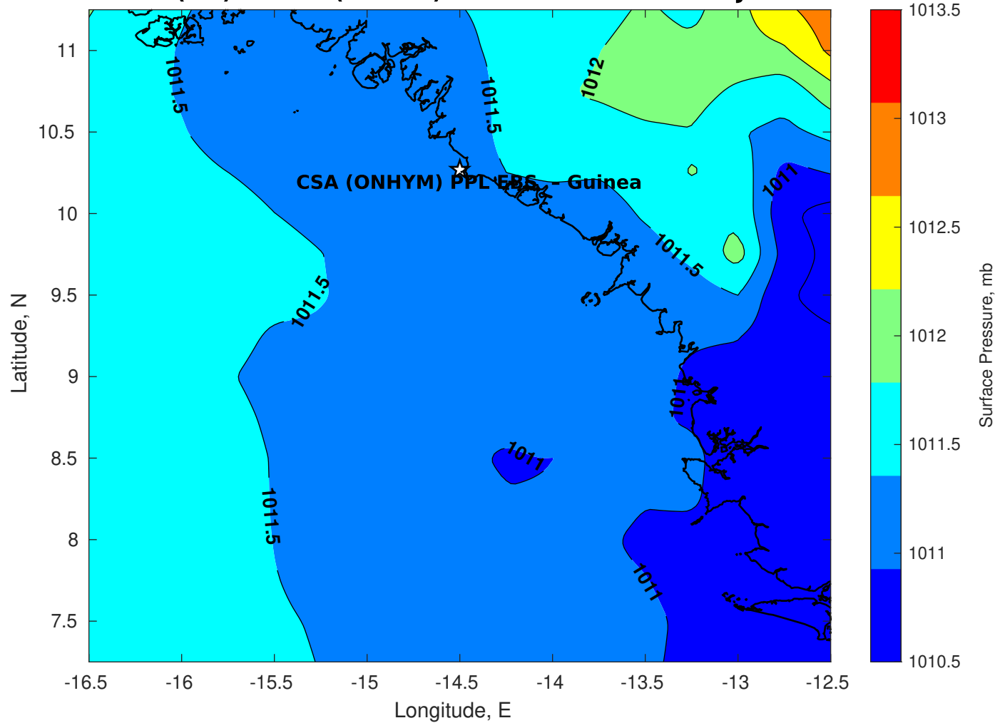
Surface Pressure (mb) for CSA (ONHYM) PPL EBS - Guinea at 20-Jan-2026 00:00:00
