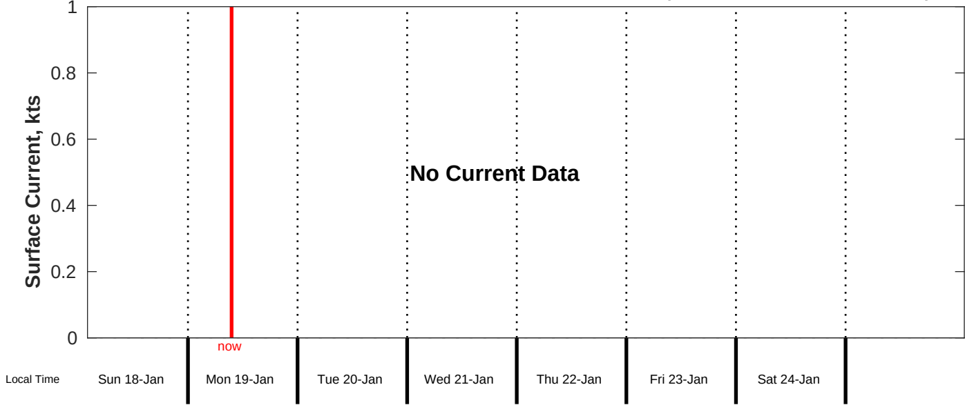
Surface Current Forecast for CSA (ONHYM) PPL EBS - Guinea from 18-Jan-2026 00:00:00 to 26-Jan-2026 00:00:00
