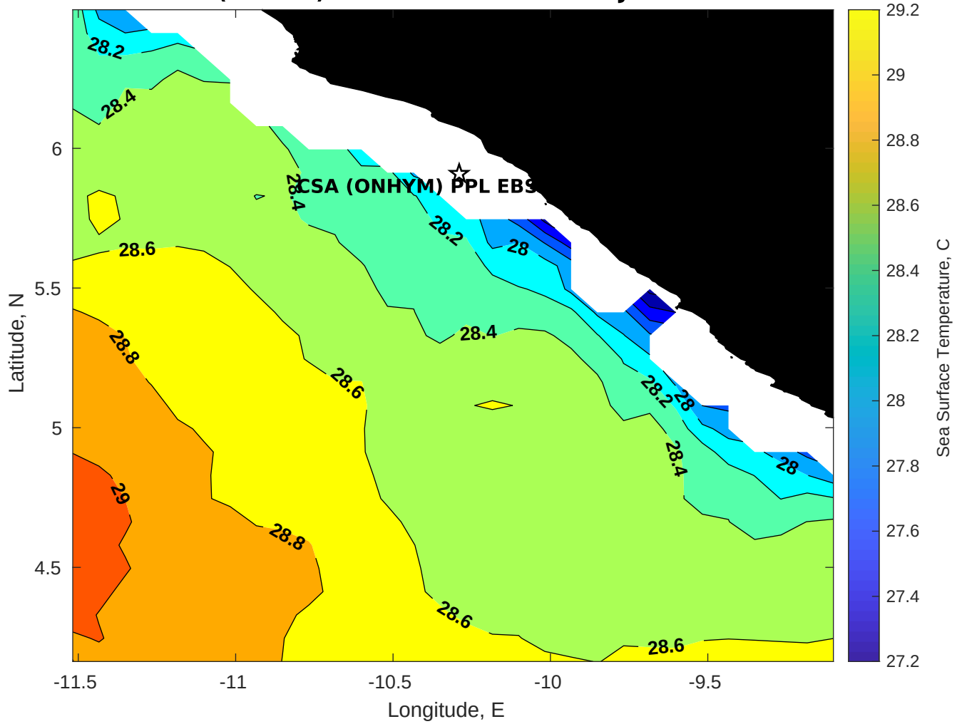
SST for CSA (ONHYM) PPL EBS - Liberia at 18-Jan-2026 00:00:00
