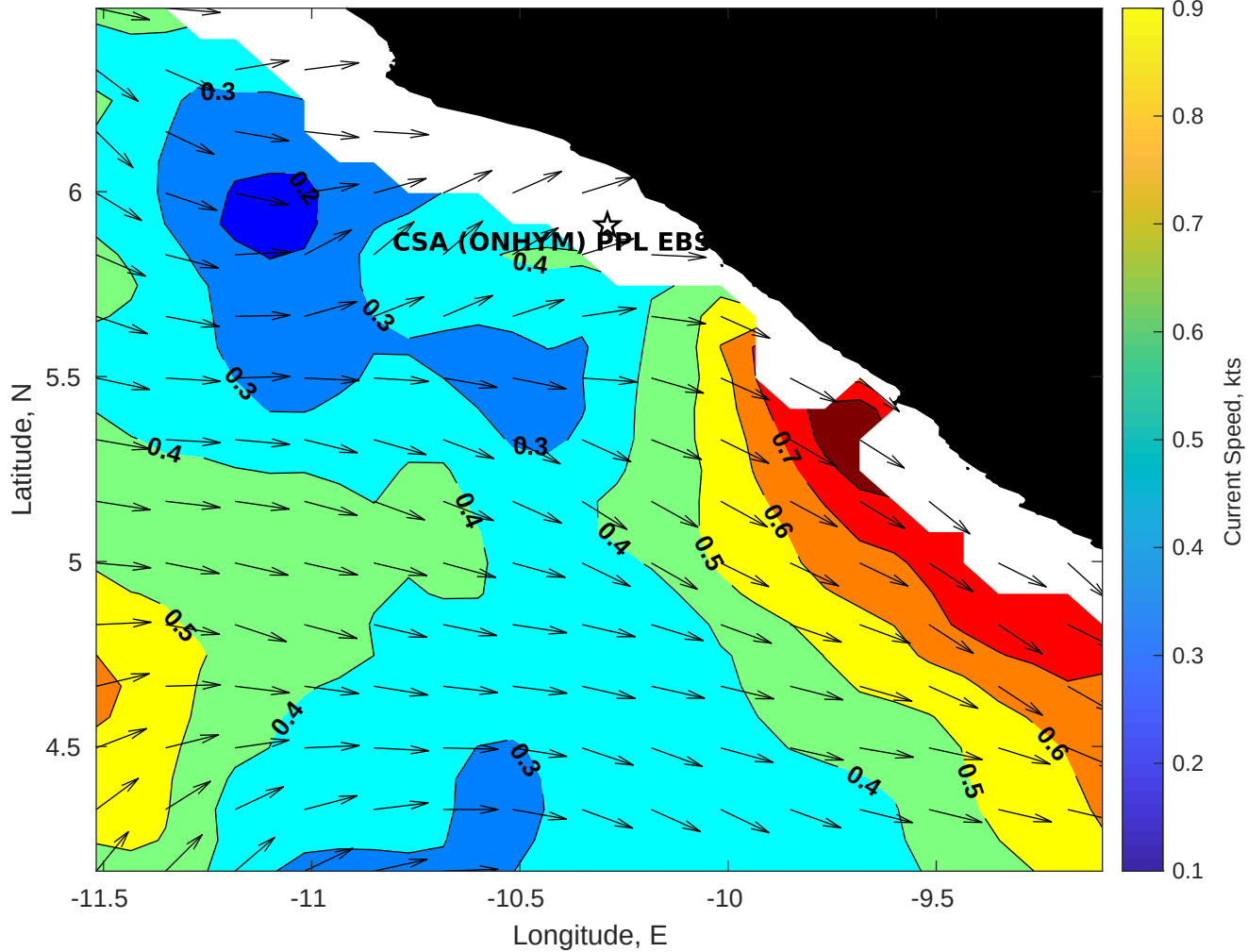
Surface Currents for CSA (ONHYM) PPL EBS - Liberia at 18-Jan-2026 00:00:00
