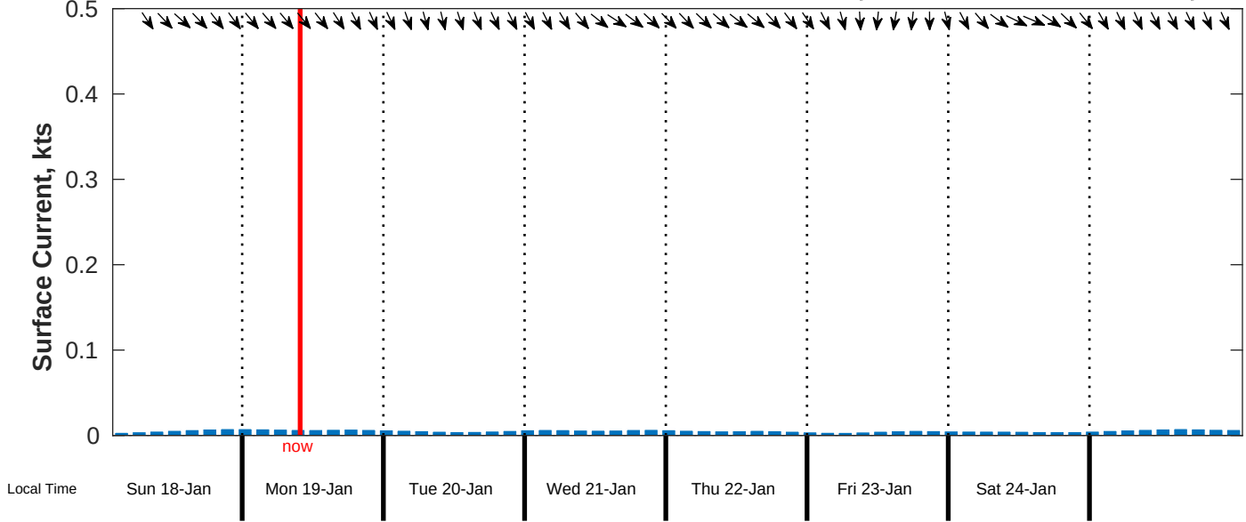
Surface Current Forecast for CSA (ONHYM) PPL EBS - Liberia from 18-Jan-2026 00:00:00 to 26-Jan-2026 00:00:00
