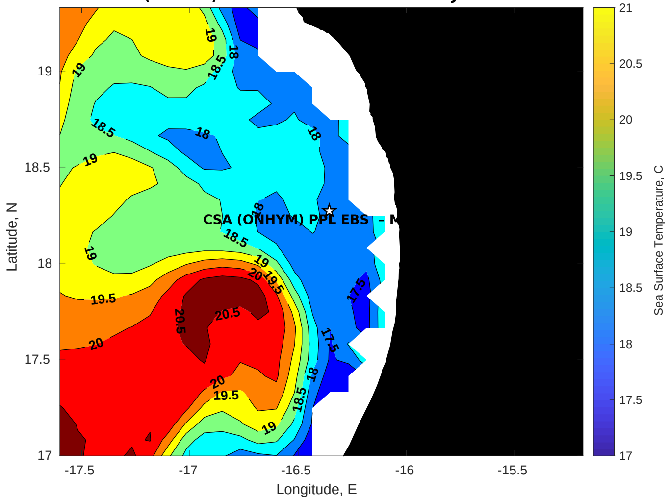
SST for CSA (ONHYM) PPL EBS - Mauritania at 18-Jan-2026 00:00:00
