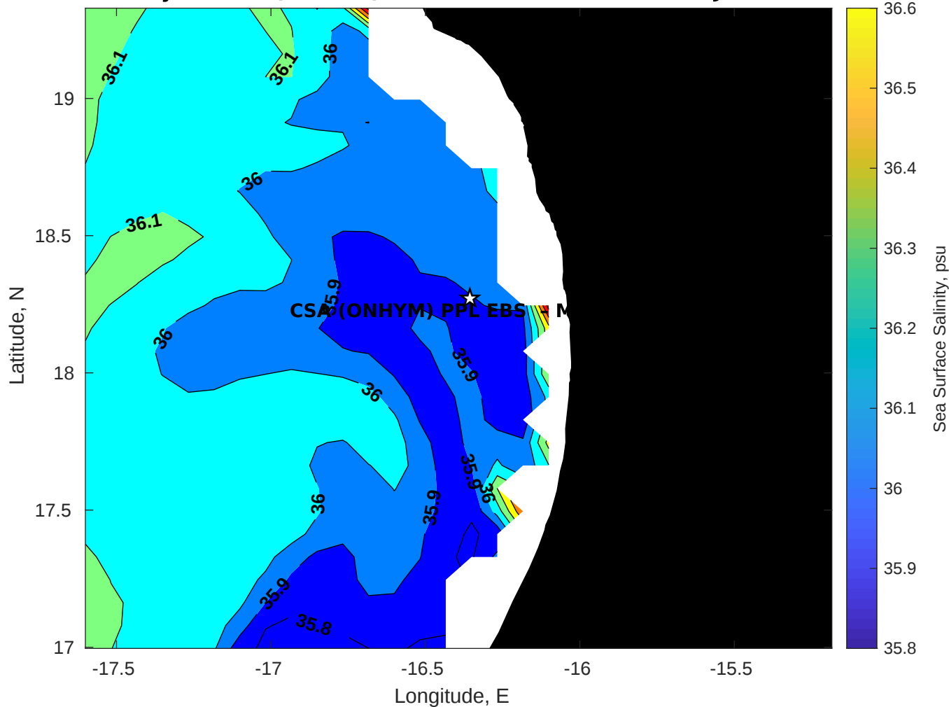
Surface Salinity for CSA (ONHYM) PPL EBS - Mauritania at 18-Jan-2026 00:00:00
