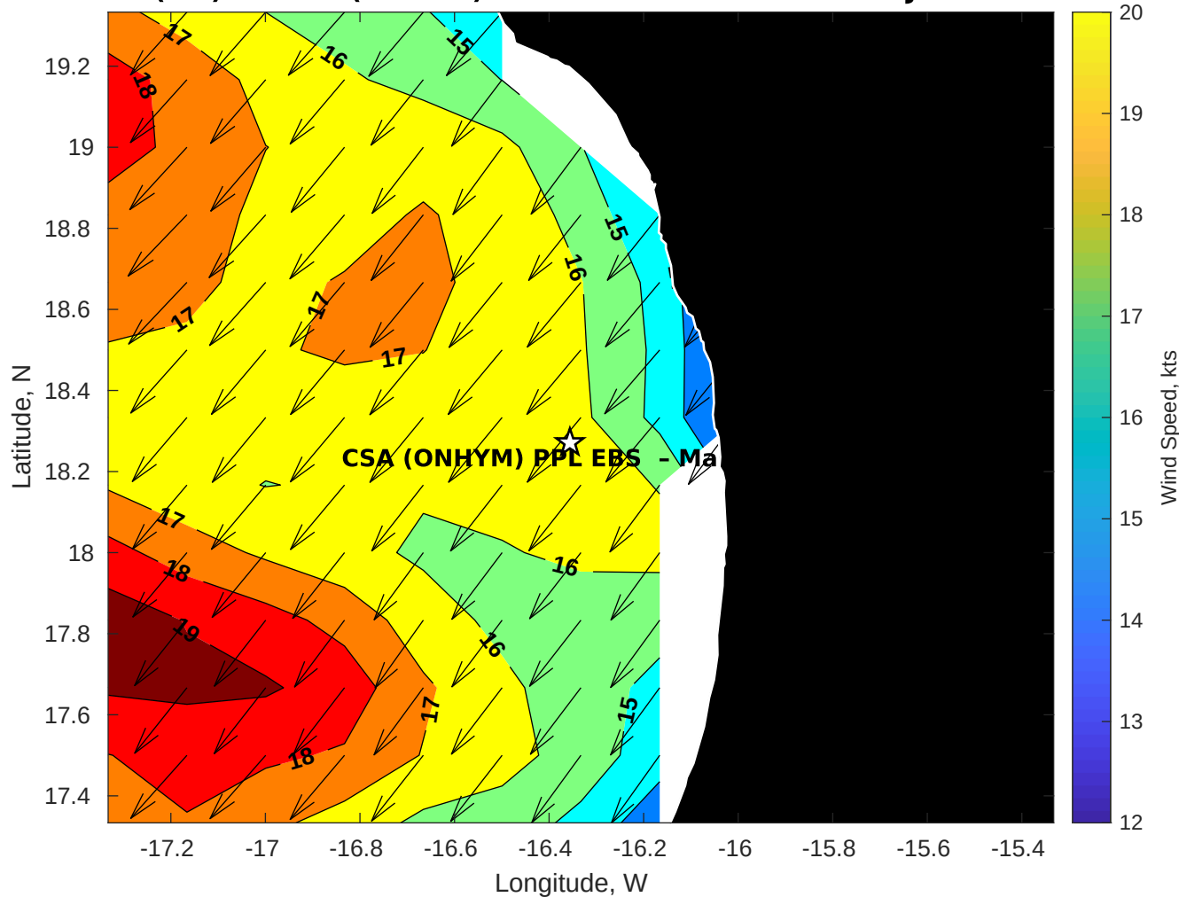
GFS Winds (kts) for CSA (ONHYM) PPL EBS - Mauritania at 19-Jan-2026 09:00:00
