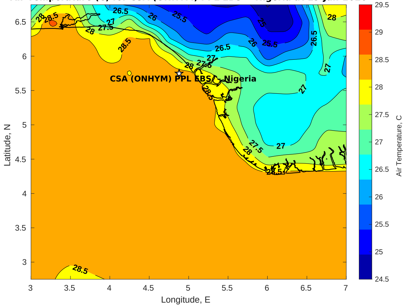
Air Temperature (C) for CSA (ONHYM) PPL EBS - Nigeria at 19-Jan-2026
