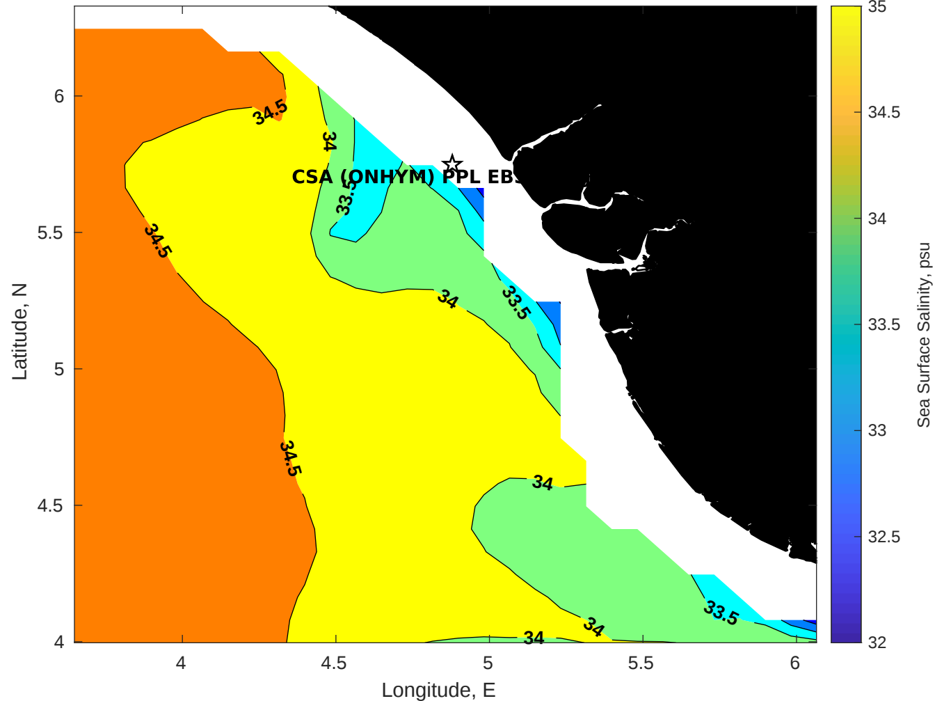
Surface Salinity for CSA (ONHYM) PPL EBS - Nigeria at 18-Jan-2026 00:00:00
