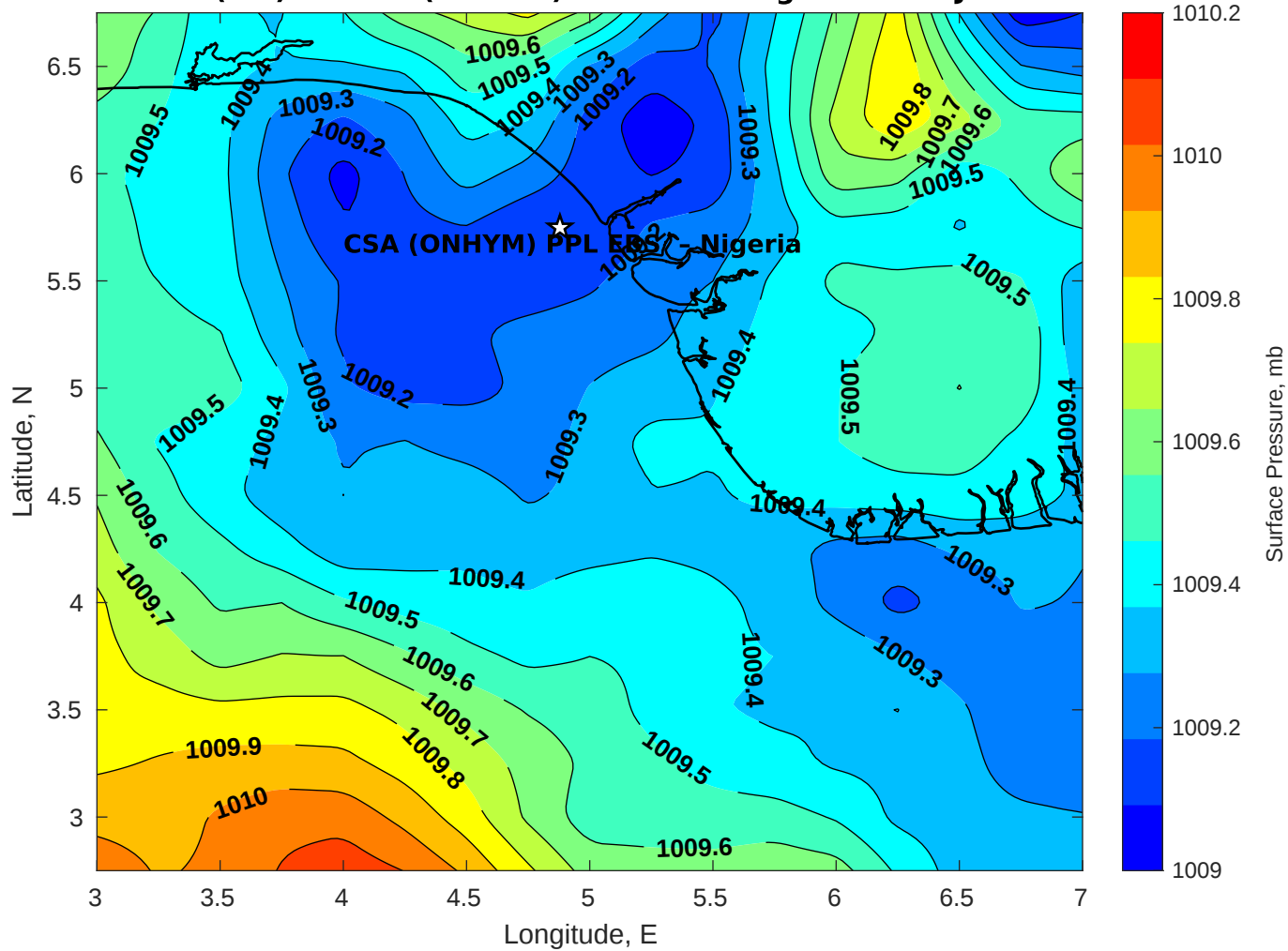
Surface Pressure (mb) for CSA (ONHYM) PPL EBS - Nigeria at 21-Jan-2026 00:00:00
