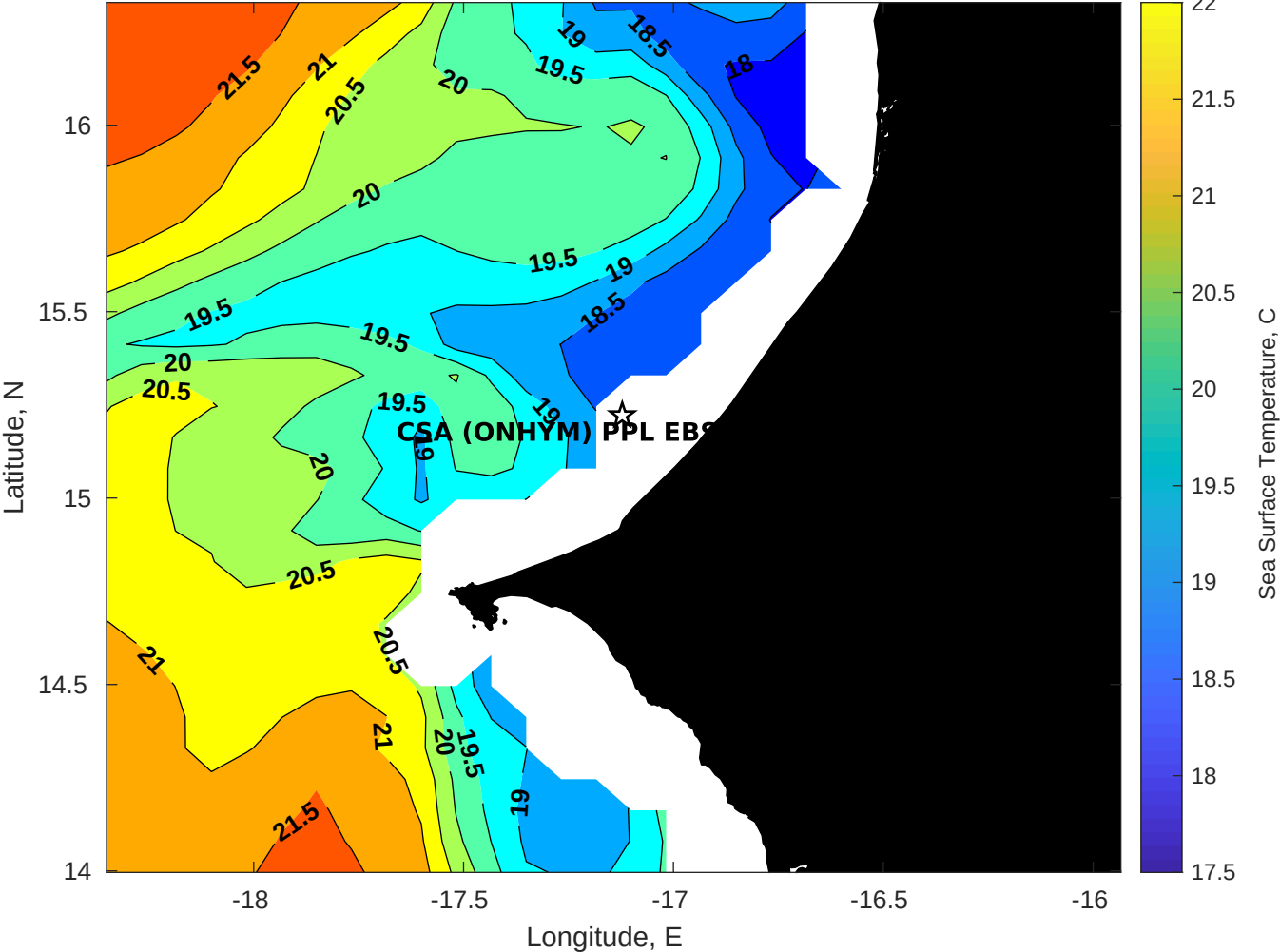
SST for CSA (ONHYM) PPL EBS - Senegal at 18-Jan-2026 00:00:00
