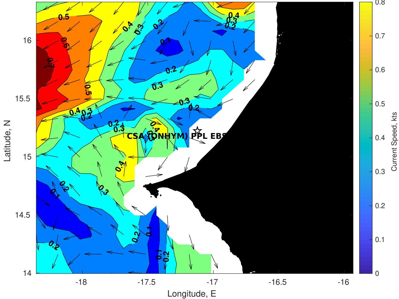
Surface Currents for CSA (ONHYM) PPL EBS - Senegal at 18-Jan-2026 00:00:00
