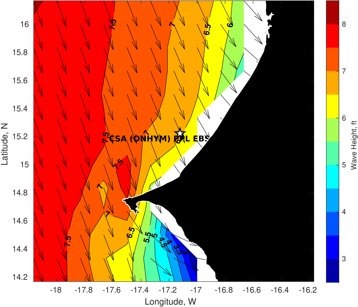
GFS Wave Height (ft) for CSA (ONHYM) PPL EBS - Senegal at 19-Jan-2026 09:00:00
