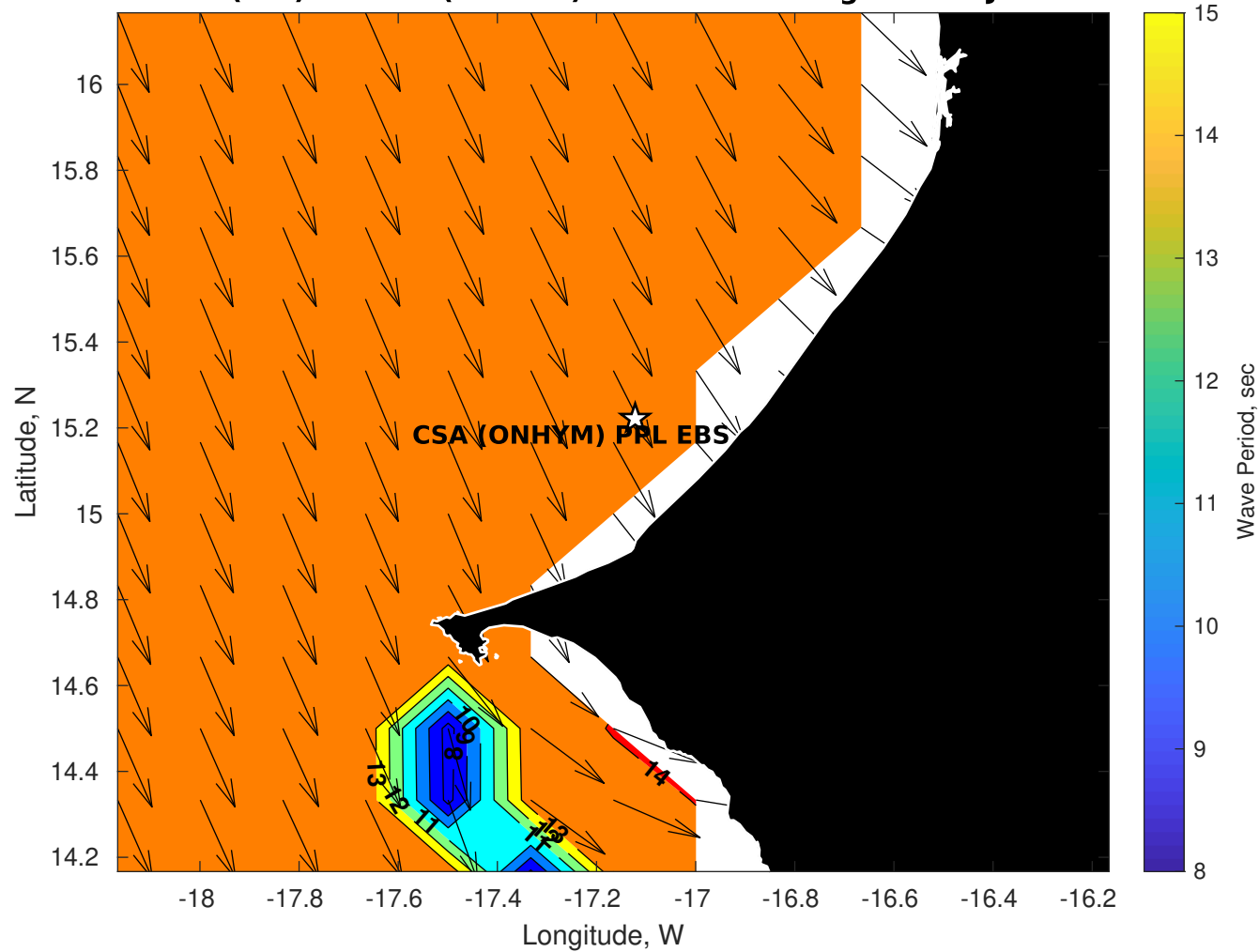
GFS Wave Period (sec) for CSA (ONHYM) PPL EBS - Senegal at 19-Jan-2026 09:00:00
