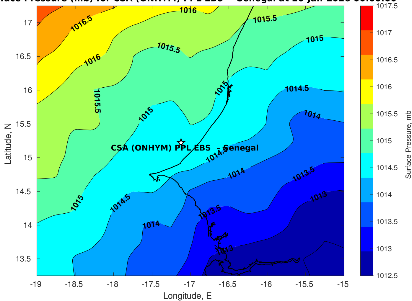
Surface Pressure (mb) for CSA (ONHYM) PPL EBS - Senegal at 20-Jan-2026 00:00:00
