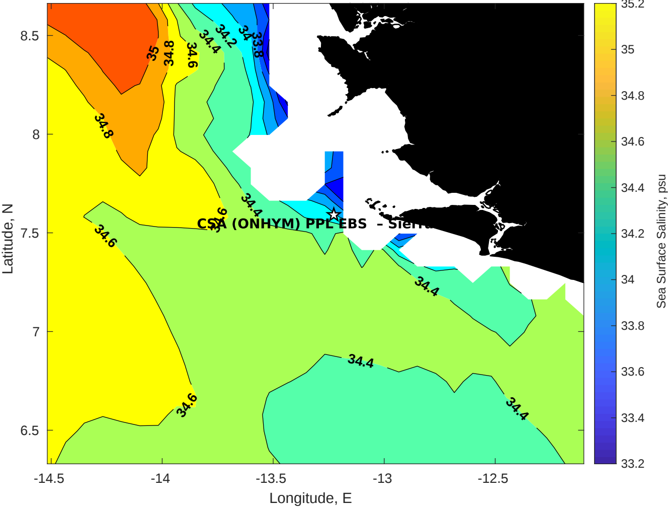
Surface Salinity for CSA (ONHYM) PPL EBS - Sierra Leone at 18-Jan-2026 00:00:00
