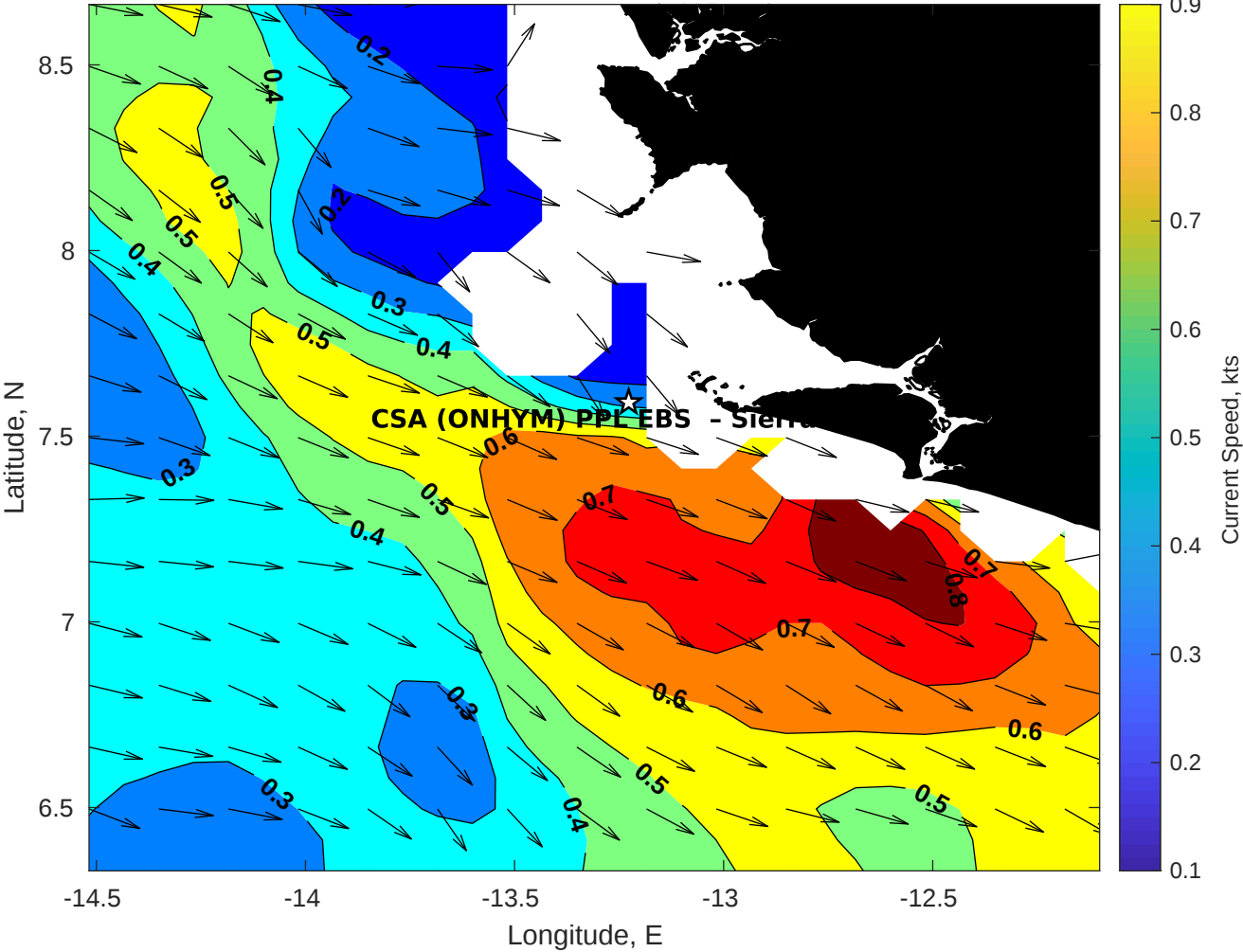
Surface Currents for CSA (ONHYM) PPL EBS - Sierra Leone at 18-Jan-2026 00:00:00
