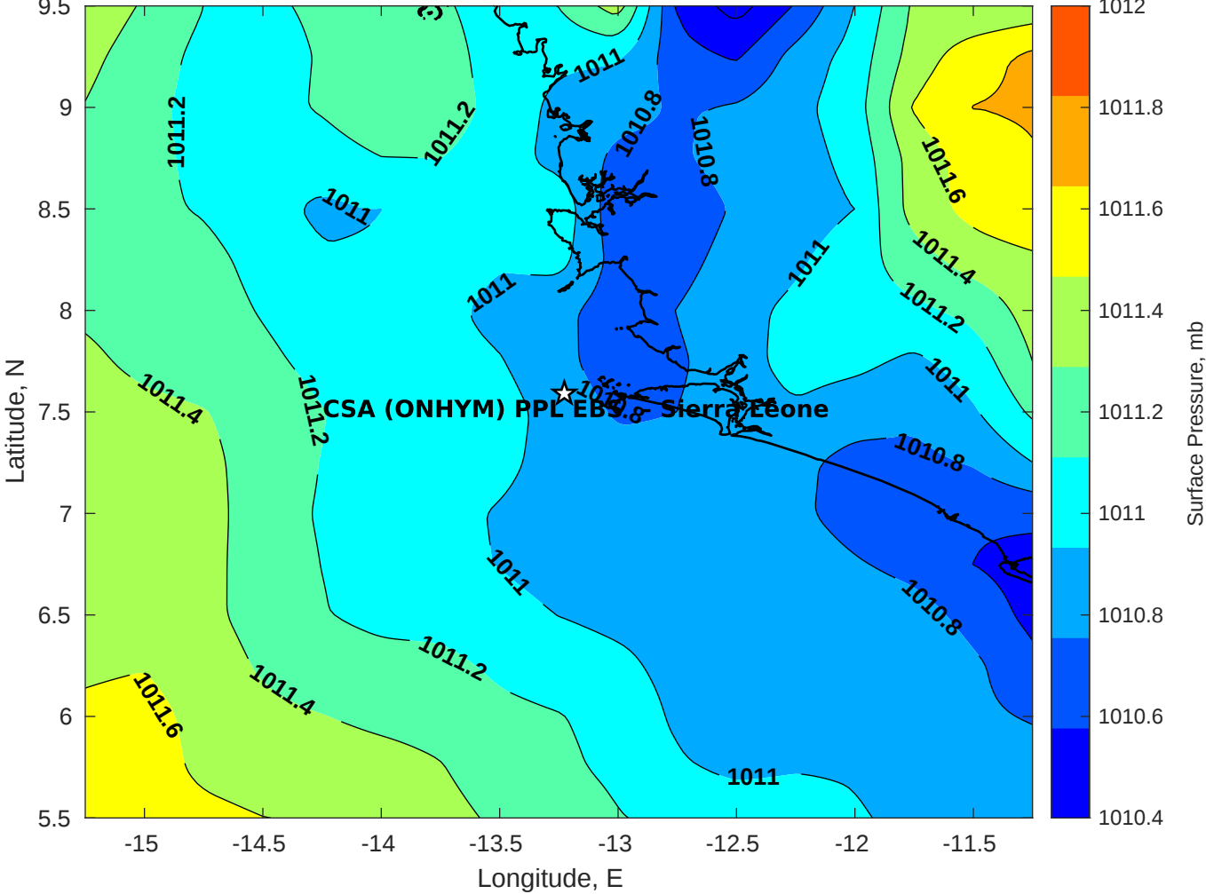
Surface Pressure (mb) for CSA (ONHYM) PPL EBS - Sierra Leone at 20-Jan-2026 00:00:00
