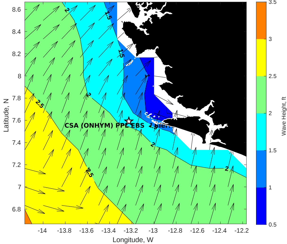
GFS Wave Height (ft) for CSA (ONHYM) PPL EBS - Sierra Leone at 19-Jan-2026 09:00:00
