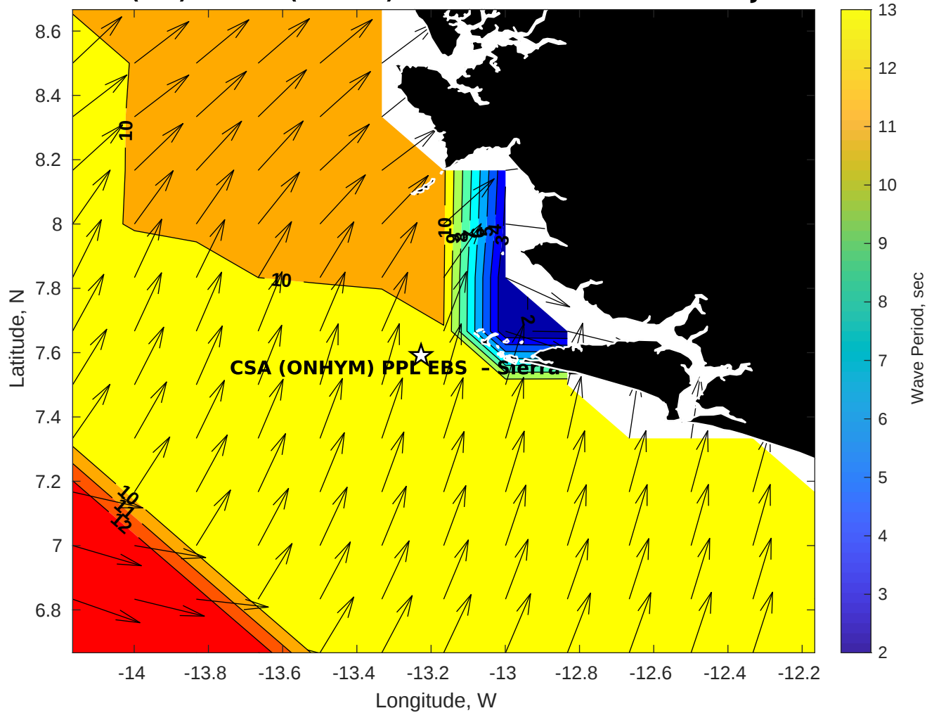
GFS Wave Period (sec) for CSA (ONHYM) PPL EBS - Sierra Leone at 19-Jan-2026 09:00:00
