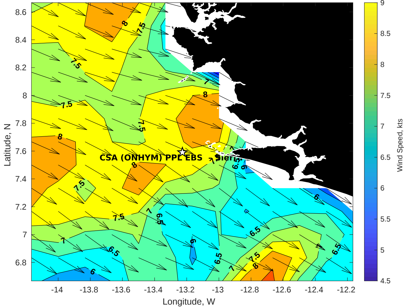
GFS Winds (kts) for CSA (ONHYM) PPL EBS - Sierra Leone at 19-Jan-2026 09:00:00
