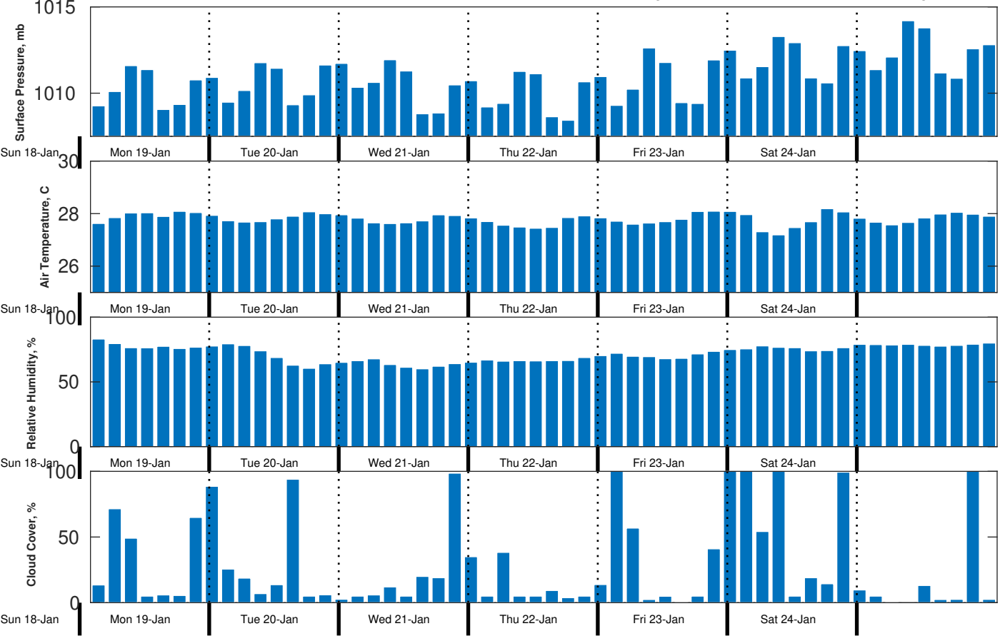
Met Forecast for CSA (ONHYM) PPL EBS - Sierra Leone from 19-Jan-2026 00:00:00 to 26-Jan-2026 00:00:00
