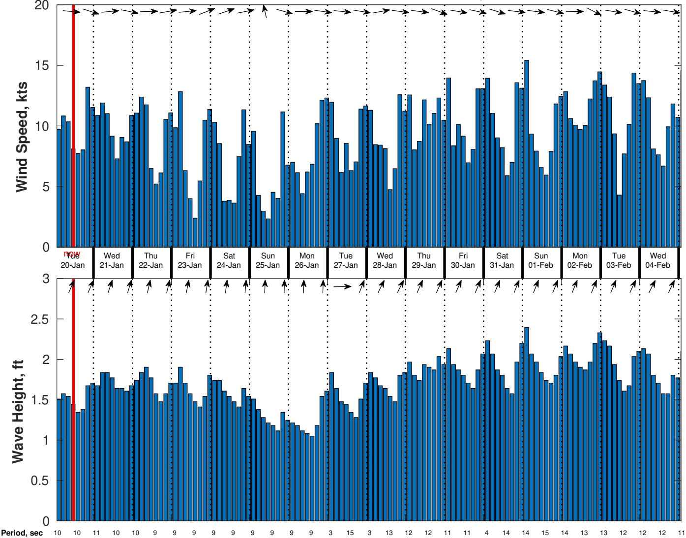
Wind & Wave Forecast for CSA (ONHYM) PPL EBS - Sierra Leone from 19-Jan-2026 01:00:00 to 04-Feb-2026 01:00:00
