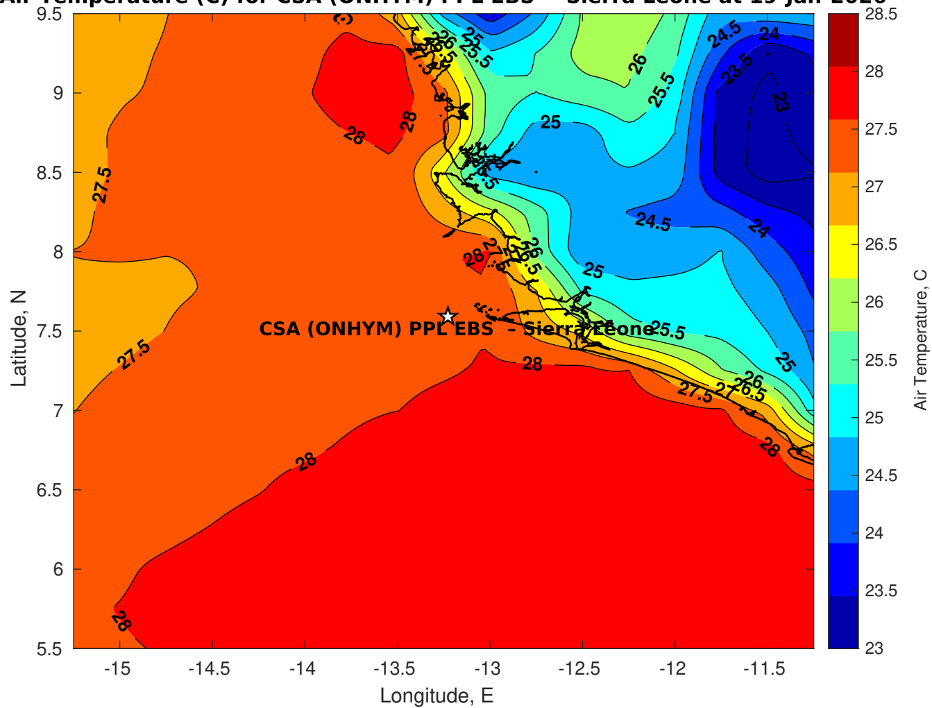
Air Temperature (C) for CSA (ONHYM) PPL EBS - Sierra Leone at 19-Jan-2026
