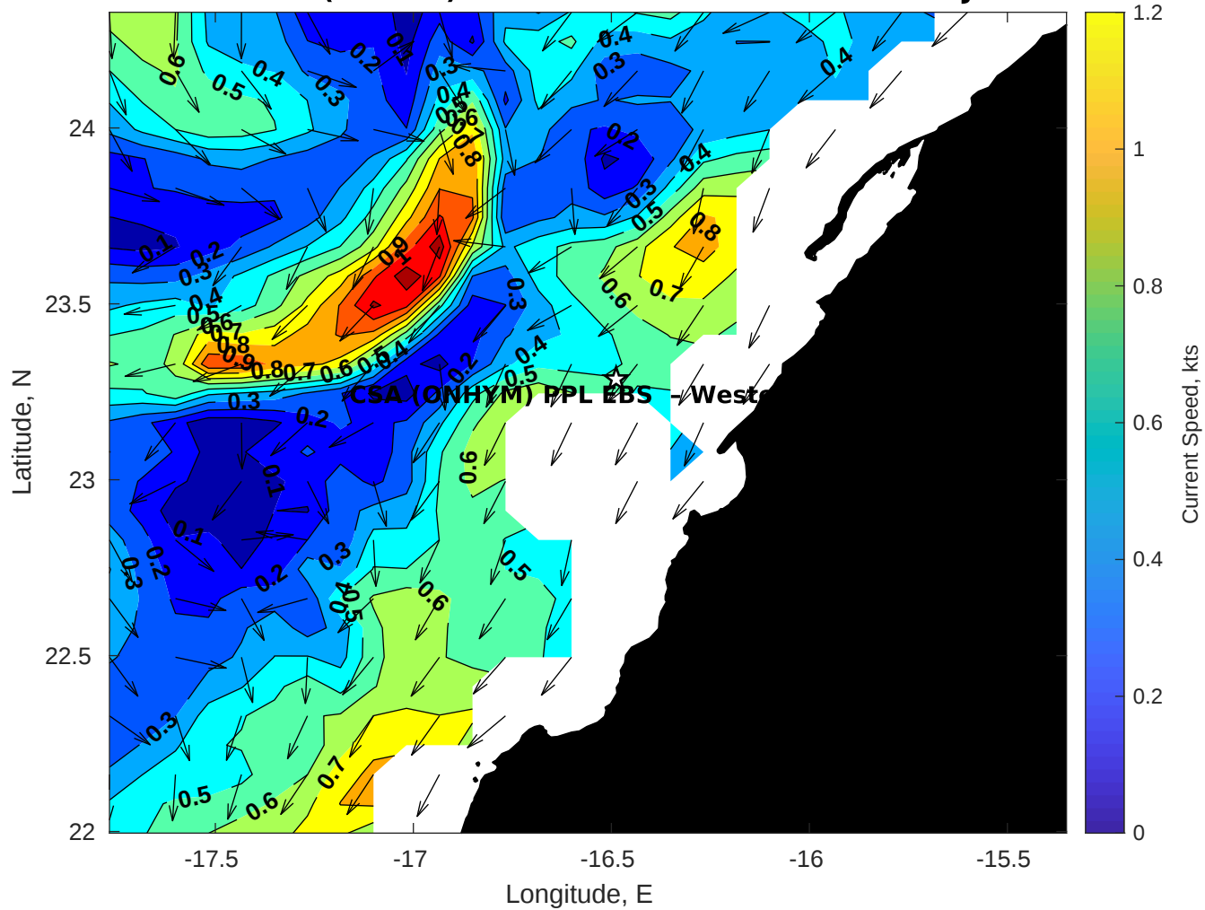
Surface Currents for CSA (ONHYM) PPL EBS - Western Sahara at 18-Jan-2026 00:00:00
